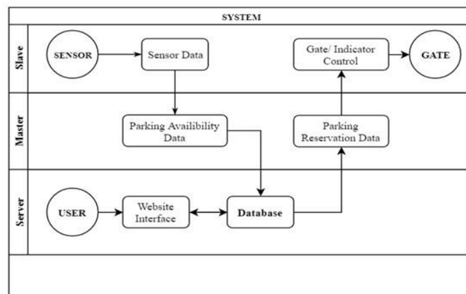
Figure 7. Flow data of the smart parking system
