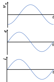
Fig. 4. Flux switching ideal waveform
