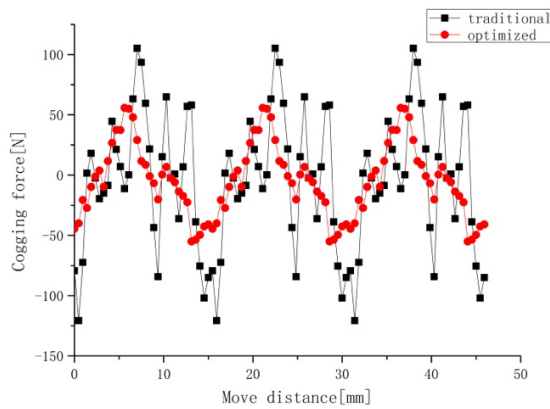
Fig. 28. Cogging force of the FSPMTM in traditional and optimized skew angle.
