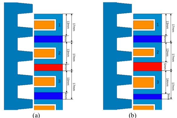
Fig. 19. Topology of the 2-D traditional FSPMTM and optimized FSPMTM.
