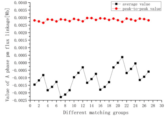
Fig. 22. Peak-to-peak value and average value of A phase pm flux linkage with different stator widths
