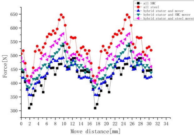
Fig. 13. Thrust force of five FSPMTM with different cores.
