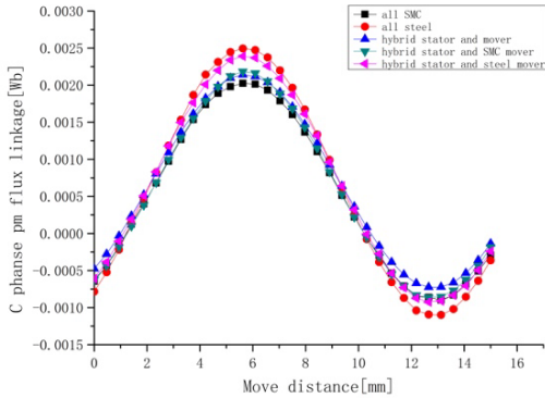
Fig. 10. PM flux linkage of the five FSPMTM.
