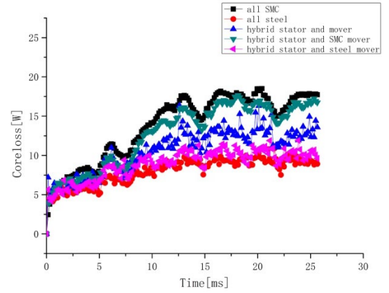
Fig. 15. Core loss comparison of FSPMTFM with different cores at load 140Hz
