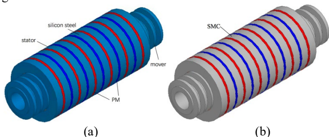
Fig. 1. Main topology of the FSPMTM, (a) M1, (b) M2.
