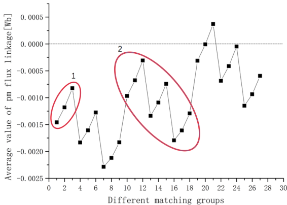
Fig. 21. Average value of A phase pm flux linkage with different stator widths
