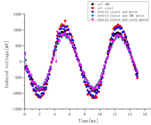
Fig. 11. Induced voltage of the five FSPMTM.
