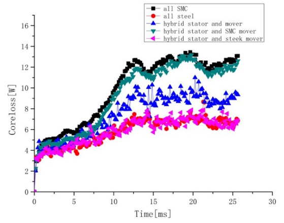
Fig. 14. Core loss comparison of FSPMTFM with different cores under no load condition.
