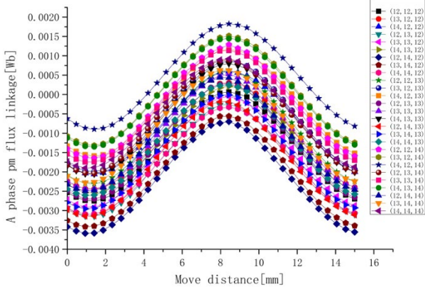
Fig. 20. Waveforms of A phase pm flux linkage with different stator widths
