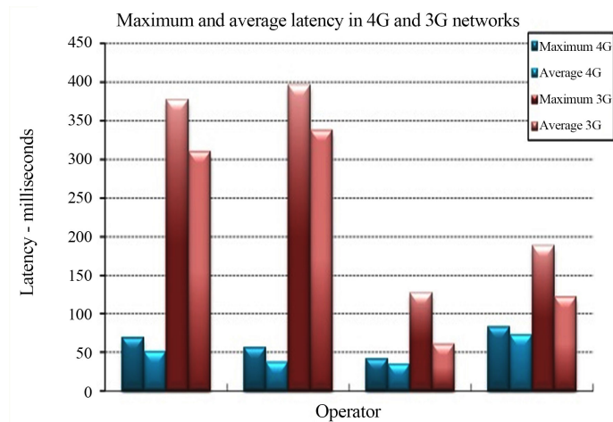
Figure 3. Maximum and average latency in 4G and 3G networks [6].
