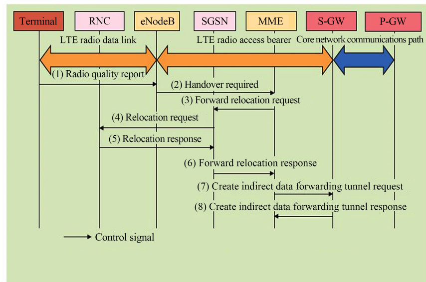
Figure 4. Preparation Procedure for Handover from LTE to 3G [7].
