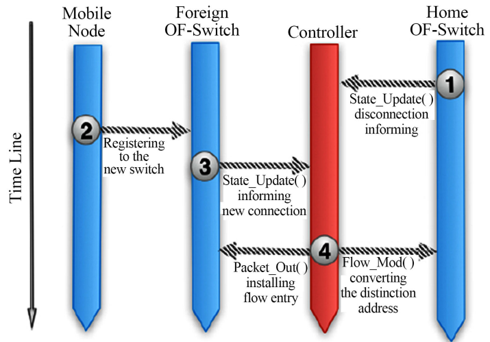
Figure 7. Registration process with OpenFlow in Mobile IP Network [10].
