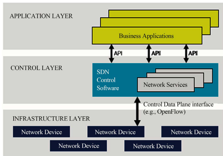
Figure 2. The SDN architecture [4].
