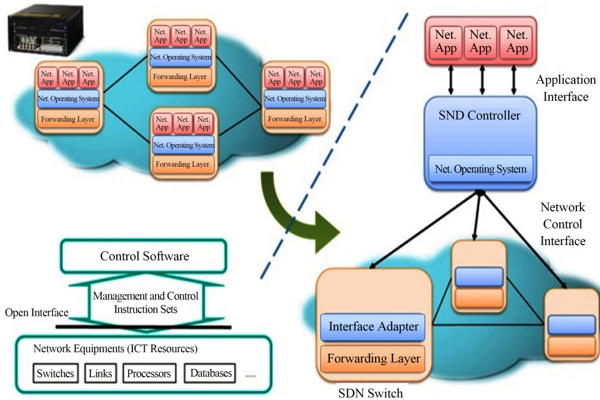
Figure 5. SDN controller and Open Flow model [8].
