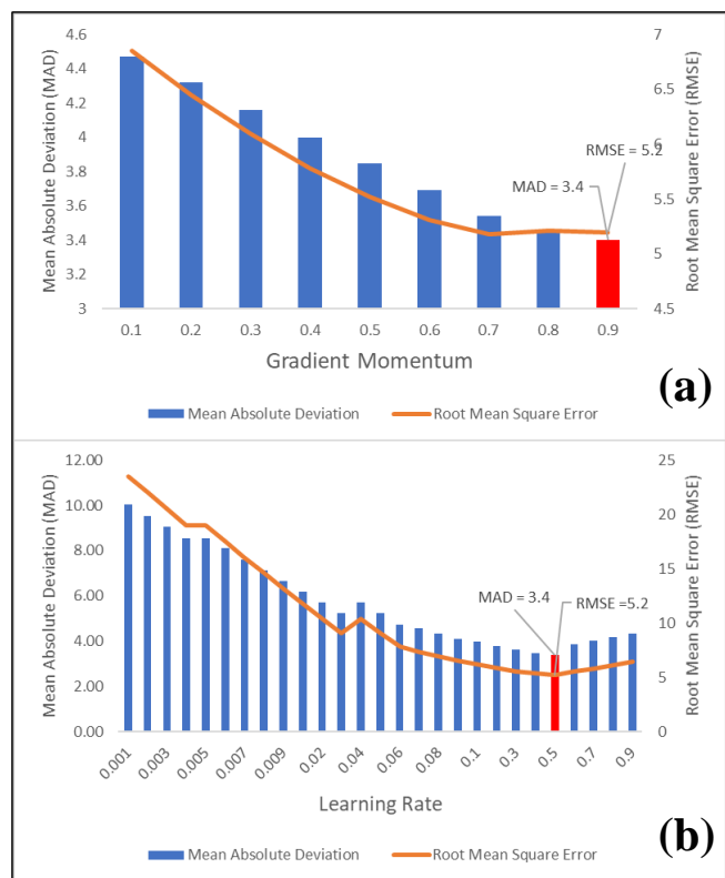
FIGURE 6. (a) The Gradient Momentum, (b) the Learning Rate with MAD and RMSE.
