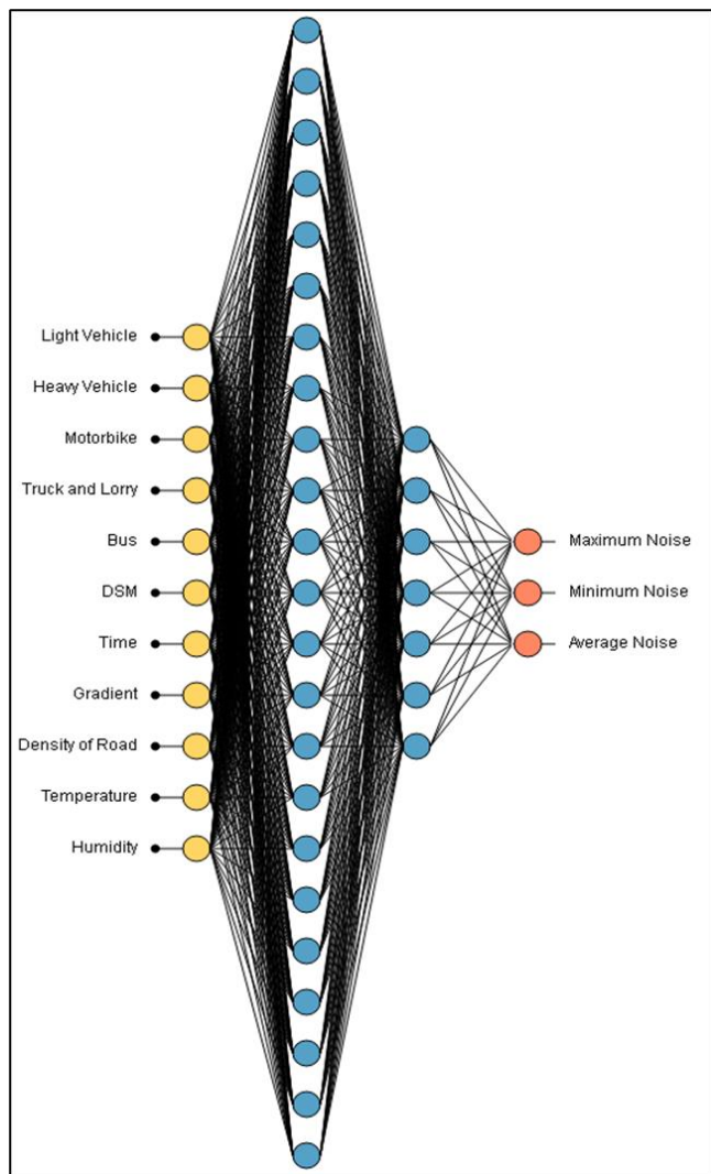
FIGURE 4. DNN architecture for predicting vehicular traffic noise (11-23-17-3)
