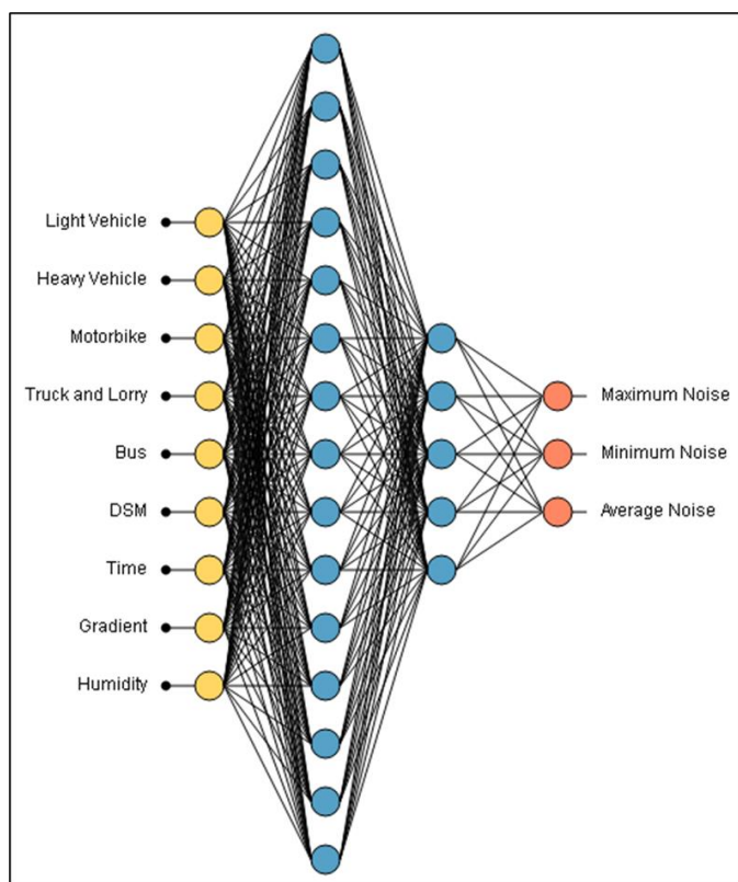
FIGURE 7. The proposed deep neural network architecture after optimising the input parameters.
