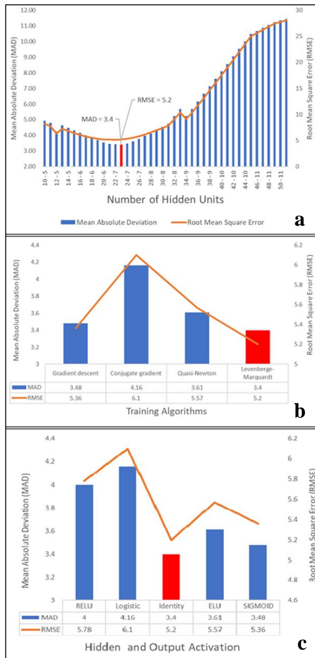
FIGURE 5. (a) The number of hidden units with MAD and RMSE, (b) The training algorithms with MAD and RMSE, (c) The hidden and output activation with MAD and RMSE.
