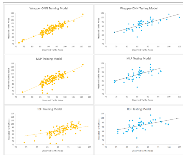
FIGURE 8. Correlation between observed and predicted vehicular traffic noise of WFS-DNN, ANN-MLP and ANN-RBF models for training and testing.
