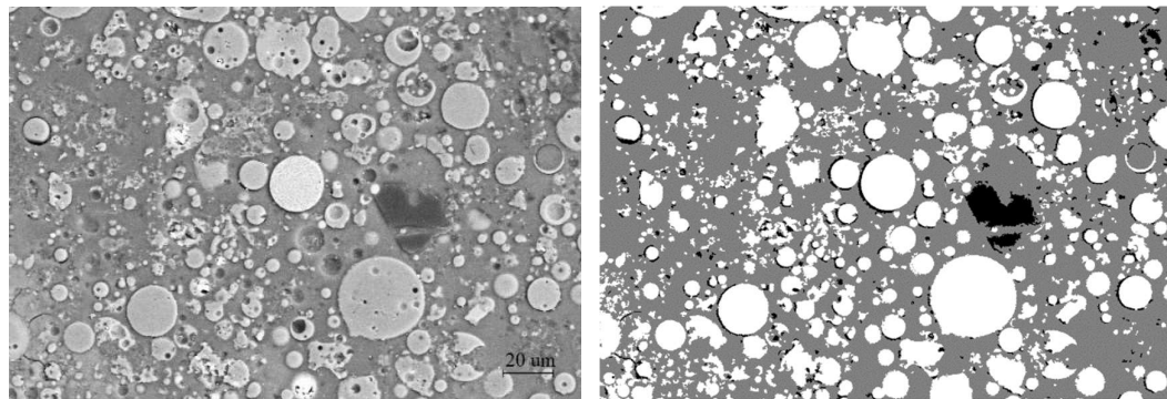
(a) BSE image (500 ×) (b) Binary image Figure 4.12 Microstructures and phase segments of AAFA based on BSE images
