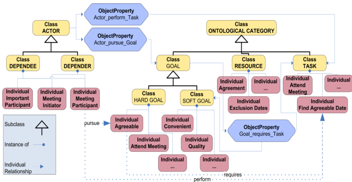
Figure 3. Excerpt of the meeting scheduler initial ontology
