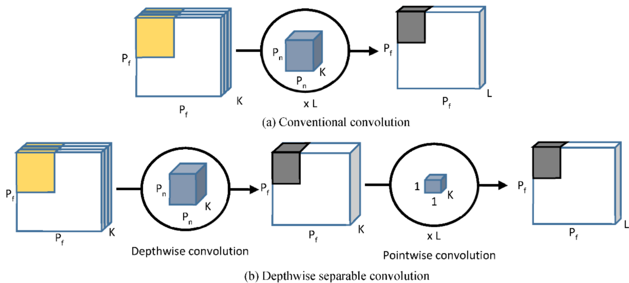
Figure 5. Schematic representation of (a) conventional vs. (b) depthwise separable convolution.
