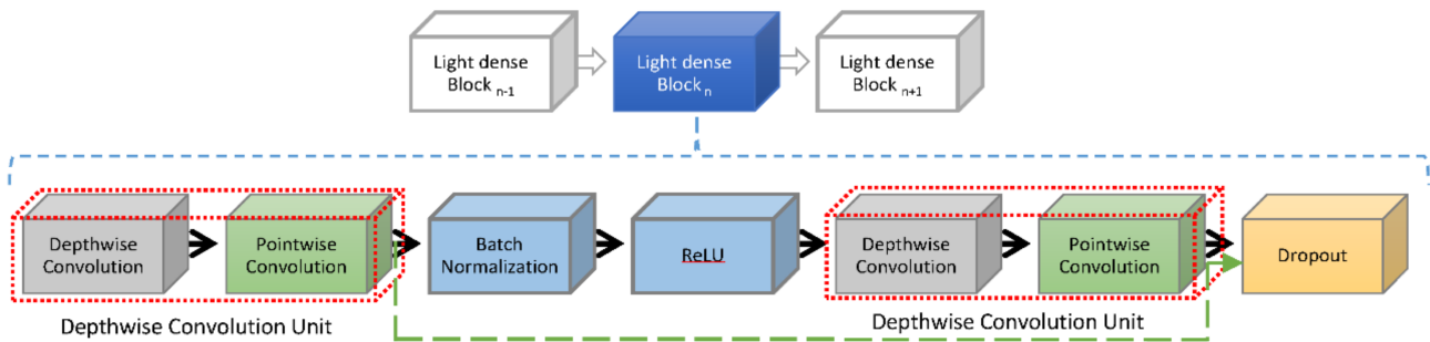
Figure 6. Proposed light dense block.
