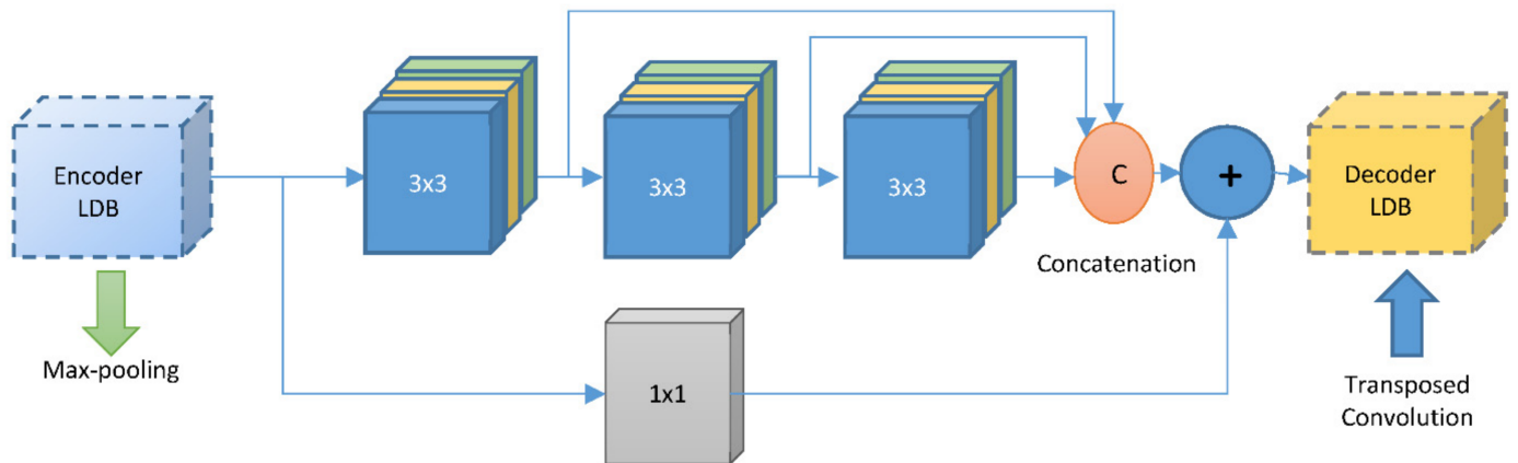
Figure 7. Multi-scale inception module.
