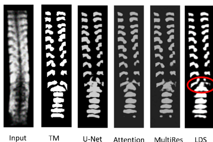
Figure 14. LDS U-Net is unable to distinguish the T12 level and 1st LBF.
