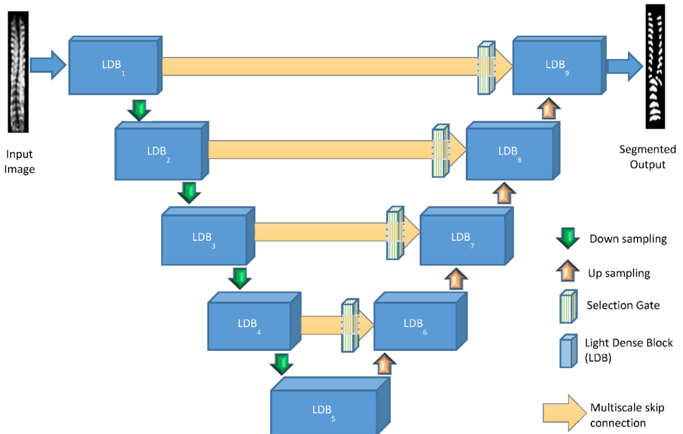
Figure 4. Proposed architecture of LDS U-Net.
