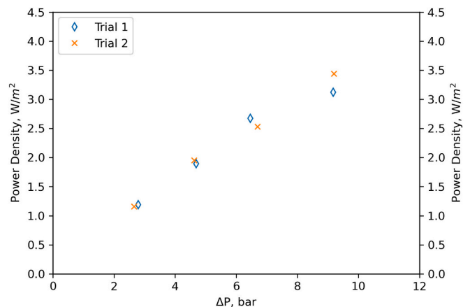
Fig. 7. Power density curve using HF membrane module with 1 M DS at 150 mL/min and DI water FS at 150 mL/min.
