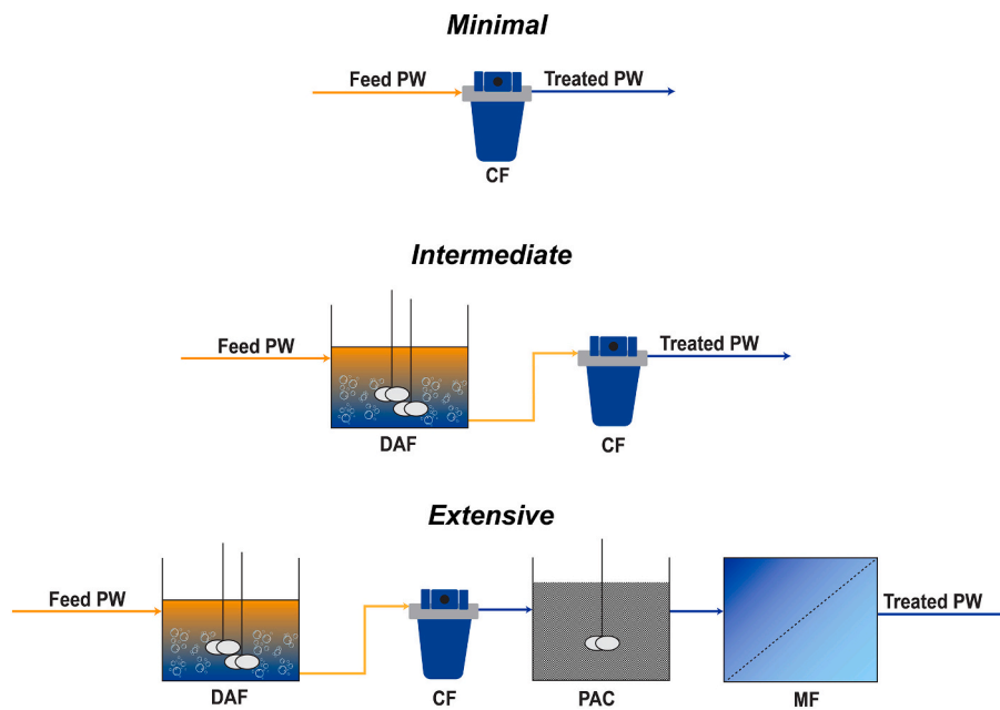
Fig. 1. Pretreatment schemes of PRO DS (actual PW).
