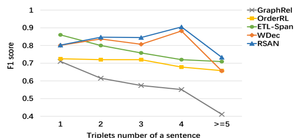
Figure 6: Relation extraction on sentences with different number of triplets.
