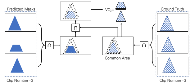
Figure 5. The pipeline for computing the video consistency. GT common area is the pixels whose GT labels are not changed in this clip. This metric is to urge predictions on these unchanged pixels to be consistent in a clip.
