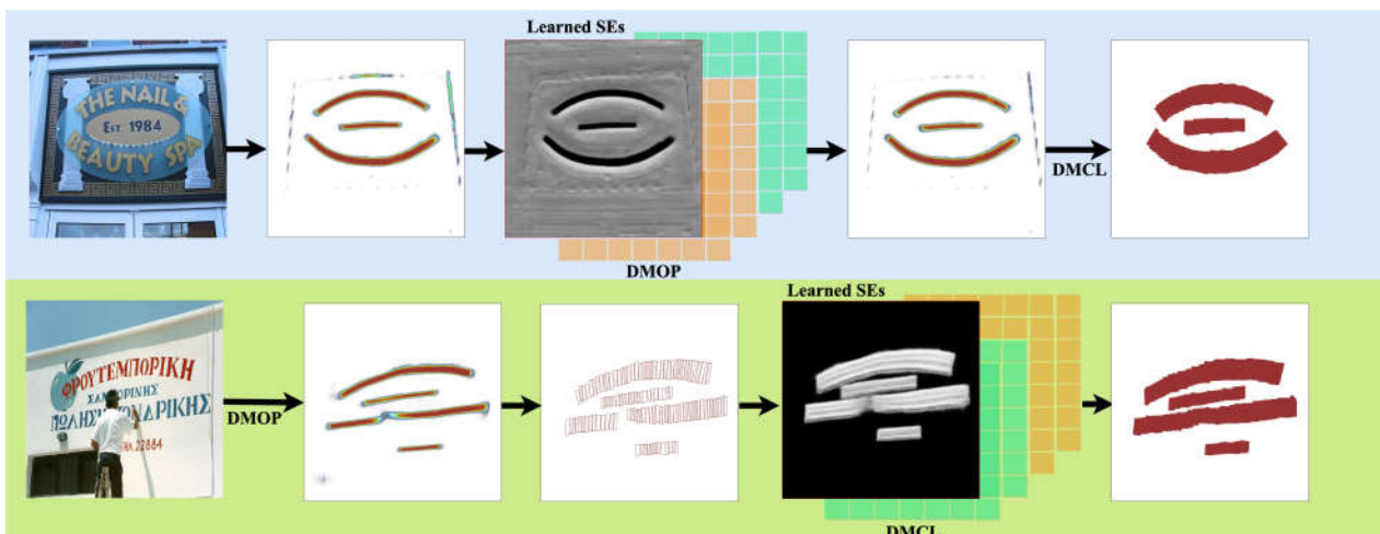
Fig. 7. Visualisation of the intermediate results of MorphText addressing noise patterns (top) and the connection problem between text segments (bottom).
