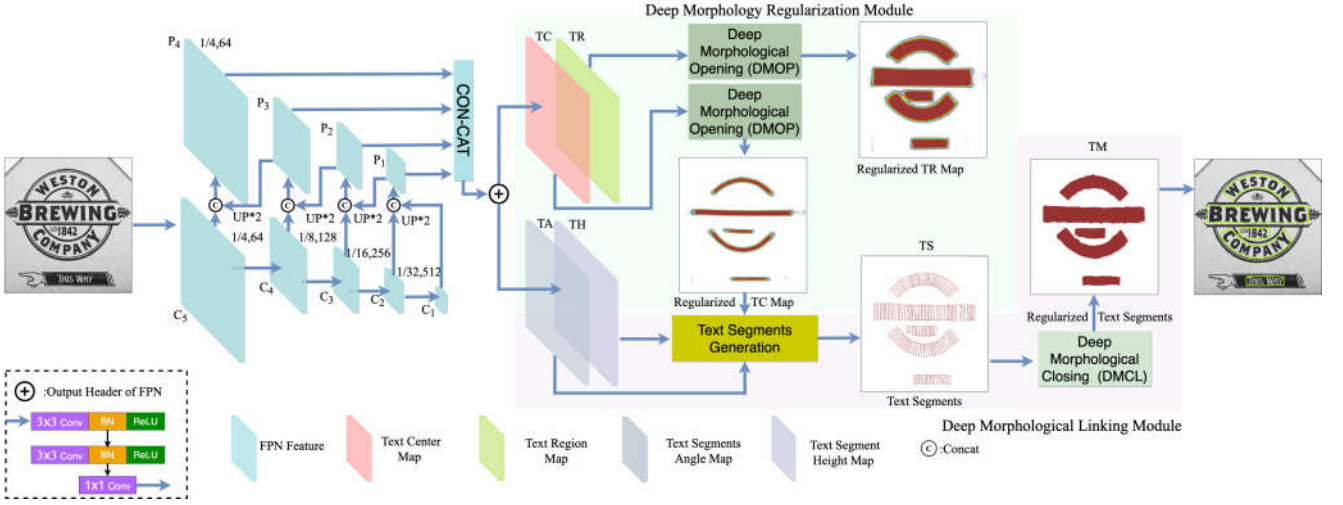
Fig. 3. The overall structure of our network, where “1/4,64”, “1/8,128”,... and “1/32,512” indicate the resize ratio and the channel number.
