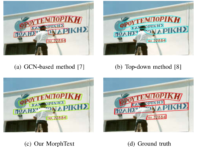
Fig. 1. Both the GCN-based method [7] and the top-down method [8] have failed (as shown in (a) and (b)) when the text instance is separated due to heavy occlusion. With our morphology regularization, such separated text segments can still be connected into a single text instance (as shown in (c)).
