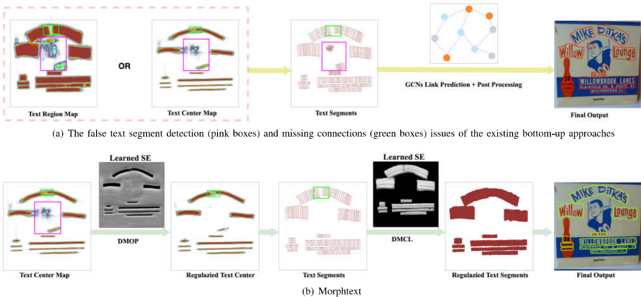
Fig. 2. Our proposed MorphText approach effectively addresses two key issues that restrain the performance of the bottom-up methods. The pink boxes indicate the false detection areas accumulated from the earlier processing and the green boxes indicate the disconnected areas.
