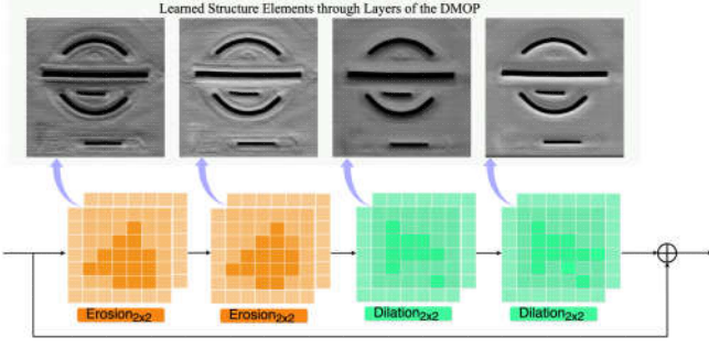
Fig. 4. The visualization of the learned structure elements through DMOP.
