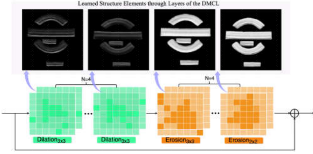
Fig. 5. Visualization of the learned structure elements through DMCL.
