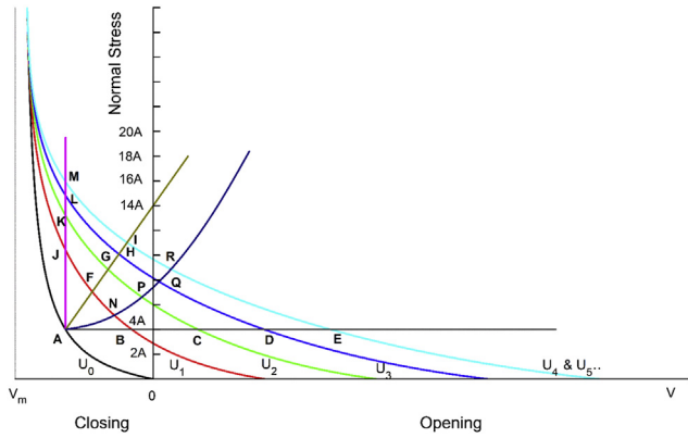
Fig. 6. Normal stress versus normal displacement at different shear displacement levels (after Saeb and Amadei, 1990).
