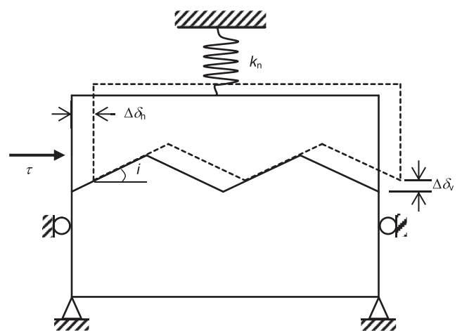
Fig. 4. Conceptual model of dilatant joints (after Heuze, 1979).
