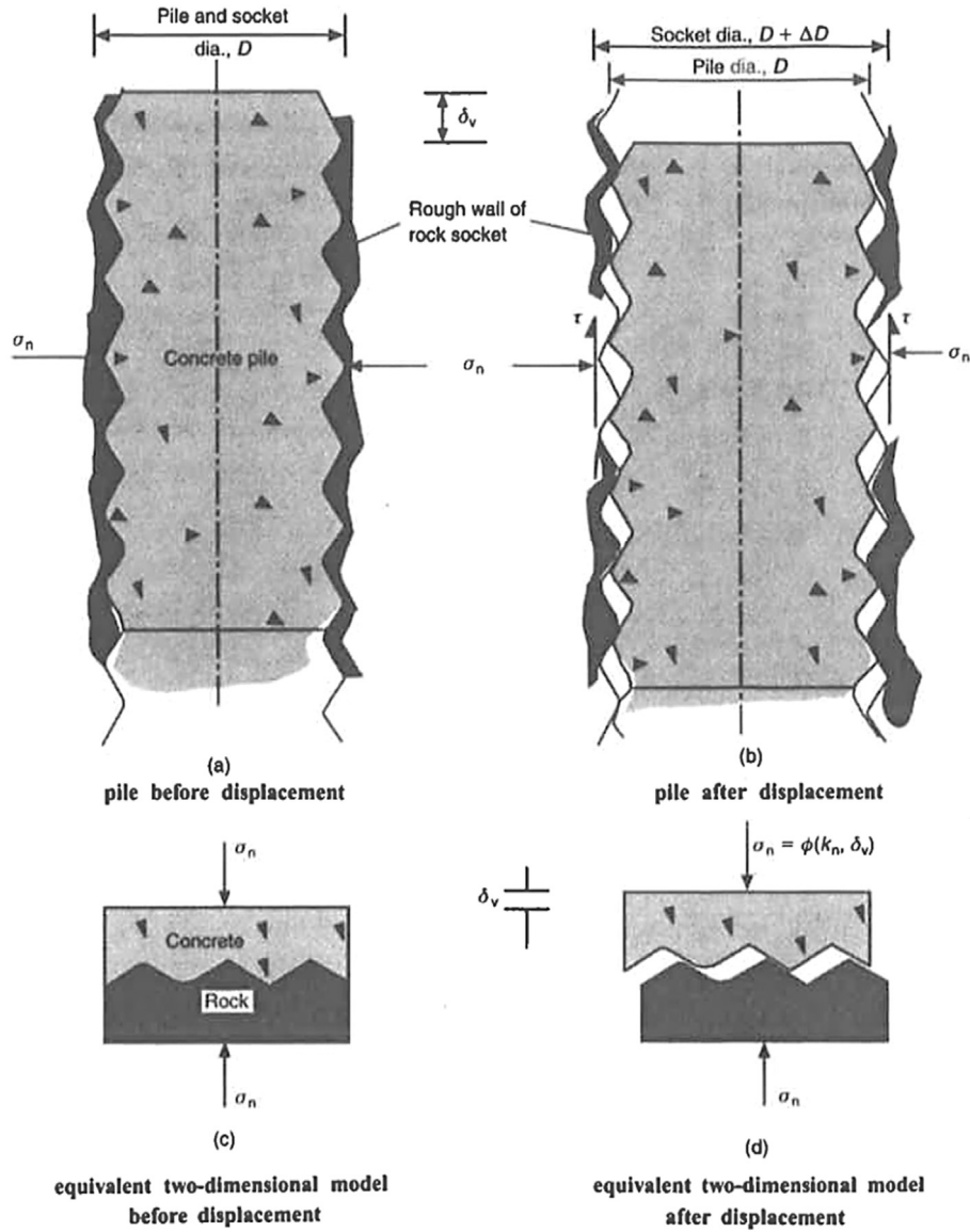
Fig. 3. Idealised displacement of pile socketed in rock (after Johnston et al., 1987).
