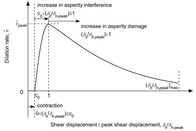
Fig. 8. A concept to model the variation of dilation rate with shear displacement (after Indraratna et al., 2015).
