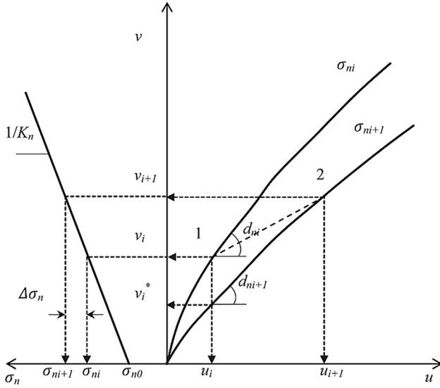
Fig. 7. The procedure for calculating dilation under CNS (modified from Skinas et al., 1990).
