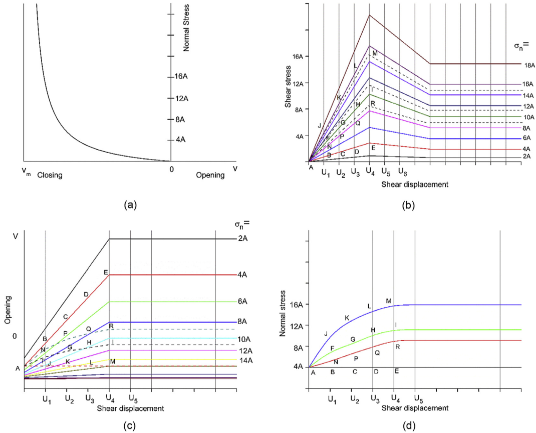
Fig. 5. The joint response curves for normal stresses ranging between 0 and 20A, where A is an arbitrary stress (after Saeb and Amadei, 1990).
