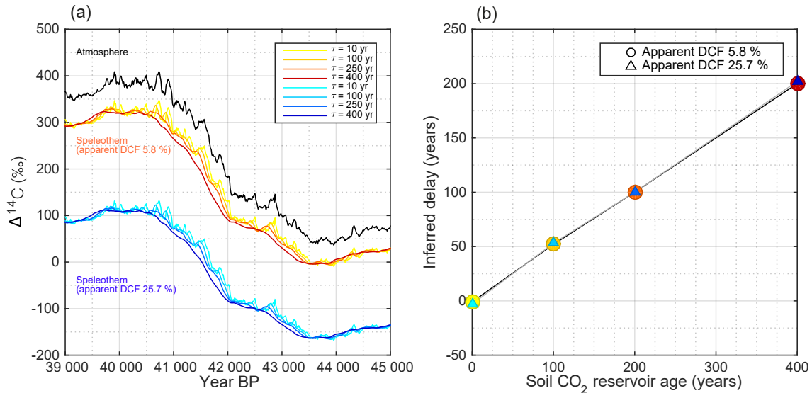
Figure 6. Effect of varying ages of soil respired CO 2 and fractions of CO 2 from 14 C dead carbonate on the Δ 14 C in speleothems. (a) Atmospheric modeled Δ 14 C from the 10 Be stack (black) and two modeled speleothem scenarios with a net DCF of 5.8 % (warm colors) and 25.7 % (cold colors). For each speleothem, a number of different ages for the respired soil organic matter have been assumed (see legend) and the input of 14 C-free CO 2 from carbonate has been adjusted to obtain the correct apparent DCF value between 39 and 40.5 ka BP. (b) The inferred delay when we apply our synchronization method to match the atmospheric Δ 14 C to the speleothem record.
