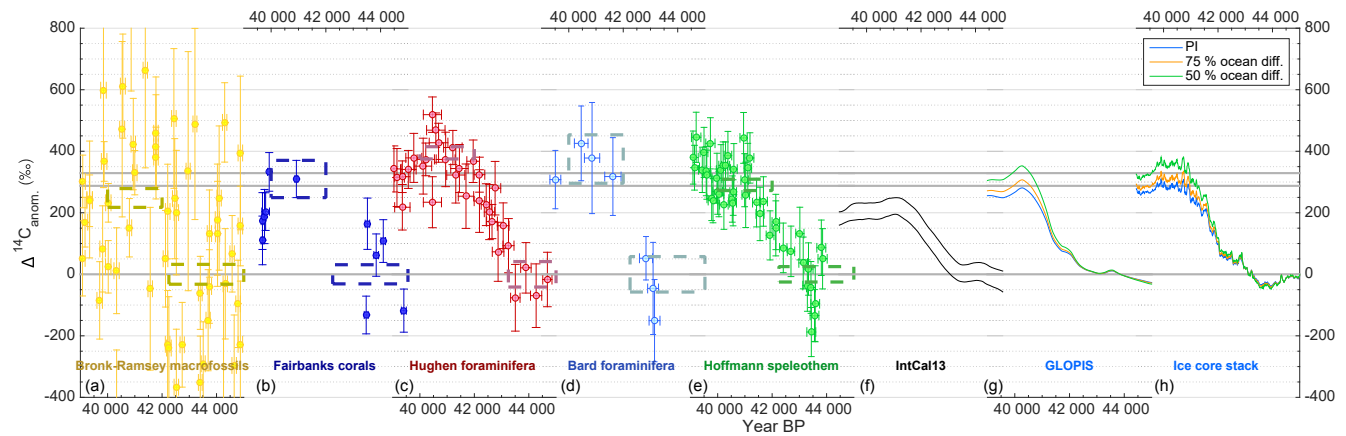
Figure 4. The Laschamp event in measured and modeled \Delta^{14}\text{C} . (a–f) \Delta^{14}\text{C} anomalies in macrofossils from Lake Suigetsu (yellow; Bronk Ramsey et al., 2012), tropical corals (blue; Fairbanks et al., 2005), foraminifera from Cariaco Basin sediments (red; Hughen et al., 2006), foraminifera from Iberian Margin sediments (light blue; Bard et al., 2013), Bahamas speleothems (green; Hoffmann et al., 2010), and IntCal13 (black; Reimer et al., 2013). All data are shown as anomalies to their error-weighted mean prior to the Laschamp event, i.e., the \Delta^{14}\text{C} increase. The dashed boxes encompass the time periods and \Delta^{14}\text{C} uncertainties (error of the error-weighted mean) used for the definition of the pre- and post-Laschamp event levels. (g, h) Modeled \Delta^{14}\text{C} using the GLOPIS (Laj et al., 2004) geomagnetic field record and the ice-core stack as production rate inputs. The different colored lines reflect different carbon cycle scenarios (see legend; PI denotes preindustrial). The conversion of geomagnetic field intensity to ^{14}\text{C} production rate is based on the production rate model by Herbst et al. (2016). Note that the amplitude of the ^{10}\text{Be} variations has been increased by 30 % as discussed in Sect. 3.3.1.
