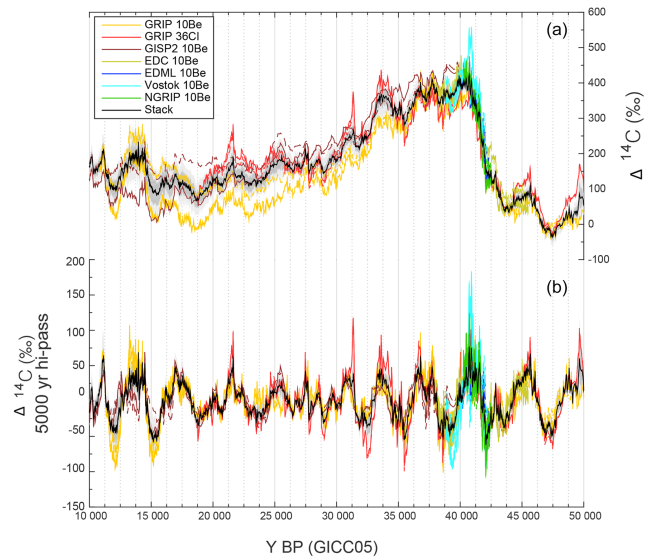
Figure 2. Modeled \Delta^{14}\text{C} anomalies from individual ice-core records (see legend; solid lines are based on radionuclide fluxes, while dashed lines are inferred from fluxes) and the realizations of the ice-core stack (black line shows the mean of all realizations, dark and light grey shading encompass 68.2% and 95.4% probability ranges). (a) The unfiltered model output. (b) The records after variations with frequencies < 1 / 5000 \text{ a}^{-1} have been subtracted (FFT-based filter).
