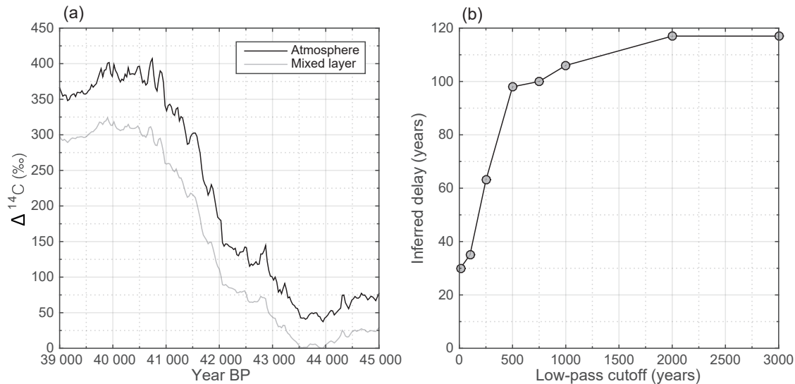
Figure 5. The delay between \Delta^{14}\text{C} in the atmosphere and ocean mixed layer. (a) Modeled \Delta^{14}\text{C} from the ice-core stack around the Laschamp event. The modeled atmospheric \Delta^{14}\text{C} is shown in black, while the ocean mixed layer is shown in grey. (b) The inferred delay from our synchronization method when comparing the atmospheric to the mixed layer signal for different low-pass filters of the mixed layer signal (x axis).
