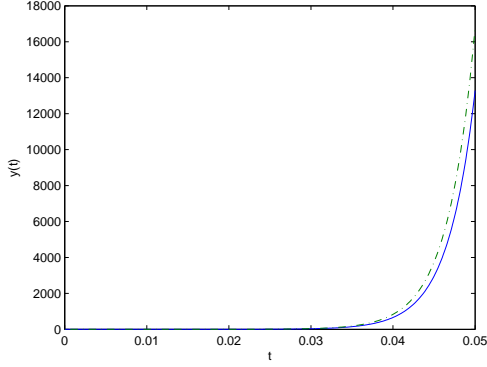
Fig. 2. Step responses of the original uncertain system \hat{G}_\Delta and the reduced system \hat{G}_{r\Delta} at \delta = 1.0 .
