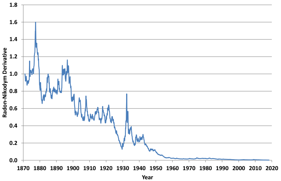
Figure 3. Plot of the sample path t \mapsto \Lambda_t of the Radon-Nikodym derivative \Lambda_t in respect of the putative risk-neutral measure.
