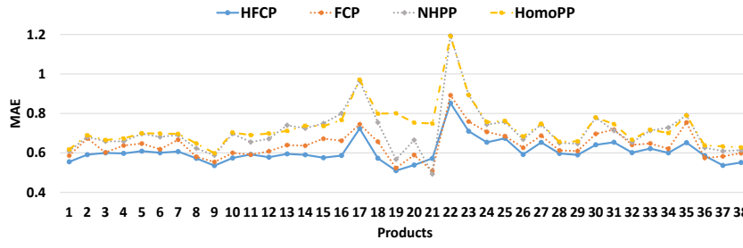
Fig. 19: MAE of the estimations of hold-out data for all products of supermarket data using HFCP, HomoPP, NHPP and FCP
