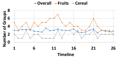
Fig. 4: Number of customer groups for all products, fruits and cereal from supermarket dataset over time (time unit is 2-week)
