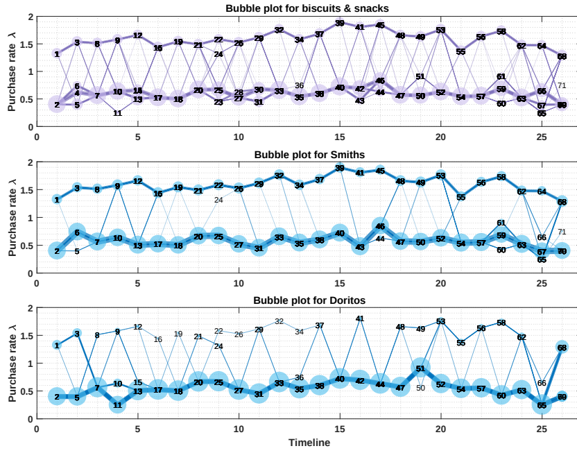
Fig. 6: Evolution of customer groups for biscuits & snacks using HFCP. The bubble plots are for the category (top), the products Smiths potato chips (middle) and Doritos potato chips (bottom)
