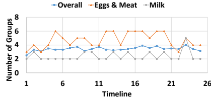
Fig. 5: Number of customer groups for all products, eggs & meat and milk from Dunnhumby dataset over time (time unit is 4-week)
