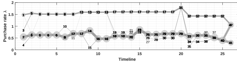
Fig. 7: Customer segmentation for the Smiths potato chips using FCP generates minor groups that overfit the data
