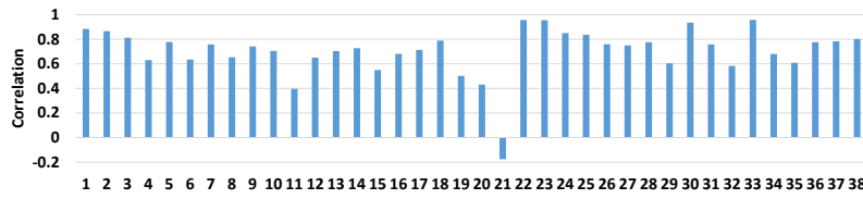
Fig. 15: Correlation of the customer distributions between a product and the category-level average for the supermarket dataset
