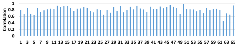
Fig. 16: Correlation of the customer distributions between a product and the category-level average for the Dunnhumby dataset
