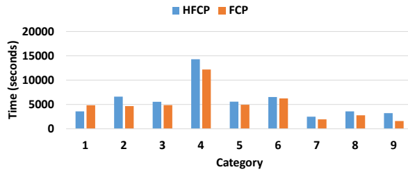
Fig. 21: Runtime of FCP and HFCP on all products from supermarket dataset
