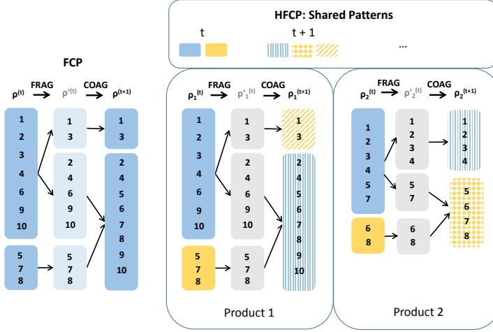
Fig. 1: Illustration of FCP (left) and HFCP for two products (right) at two time steps
