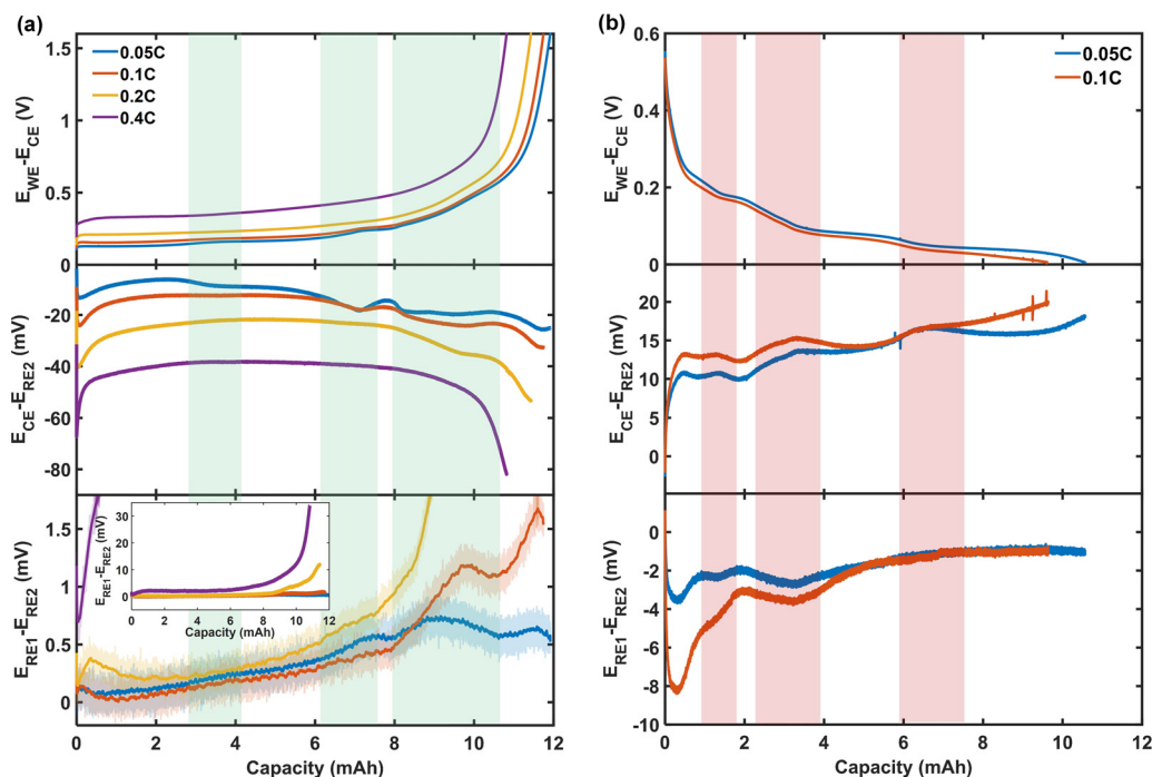
Fig. 7. (a) Various potential differences between the four electrodes during constant current charging at 0.05, 0.1, 0.2, and 0.4 C-rates ( 1C=12 mA). (b) Potential differences during discharging at 0.05 and 0.1C. The top, middle, and bottom panels show the potential differences between WE and CE, CE and RE2, and RE1 and RE2, respectively. The inset in the bottom panel of (a) shows the behavior of the potential differences on a larger scale. The green- and red-shaded areas indicate the simultaneous fluctuations between potential differences in the middle and bottom panel and the stepped regions in the top panel for charging and discharging, respectively.
