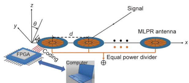
Fig. 1. Illustration of a polarization programmable antenna array. \theta : the elevation angle from the positive z -axis; \phi : the azimuth angle from the positive x -axis; d : the element spacing.
