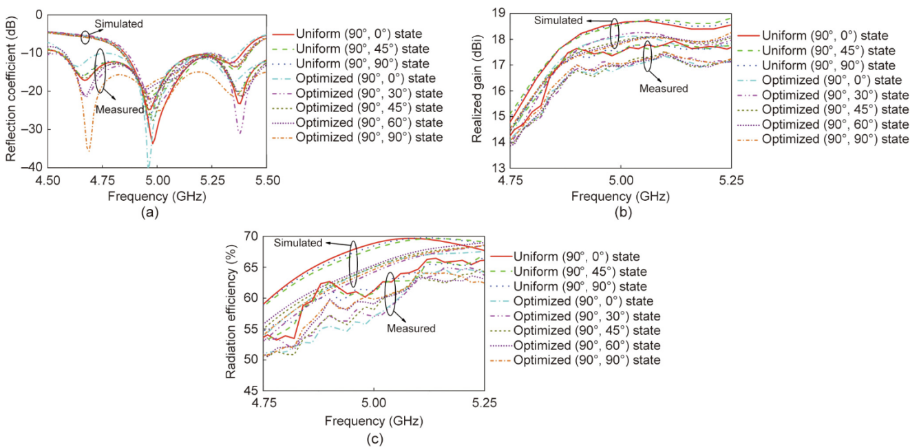
Fig. 13. The measured and simulated performances of the MLPR antenna array under the five optimized polarization state configurations and the Uniform (90°, 0°) state, Uniform (90°, 45°) state, and Uniform (90°, 90°) state. (a) Reflection coefficients; (b) realized gains; (c) radiation efficiencies.
