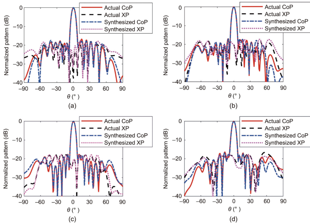
Fig. 10. The synthesized CoP and XP patterns and corresponding actual array patterns obtained by the full-wave simulation of the MLPR antenna array. (a)–(d) The obtained patterns for the desired polarization of (a) (90^\circ, 0^\circ) , (b) (90^\circ, 45^\circ) , (c) (90^\circ, 60^\circ) , and (d) (90^\circ, 90^\circ) .
