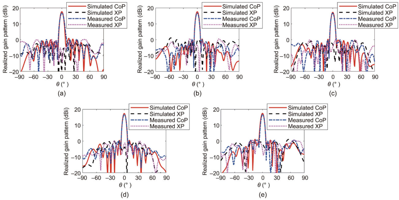
Fig. 12. The measured and simulated patterns of the MLPR antenna array when the desired polarizations are (a) (90°, 0°); (b) (90°, 30°); (c) (90°, 45°); (d) (90°, 60°); and (e) (90°, 90°).
