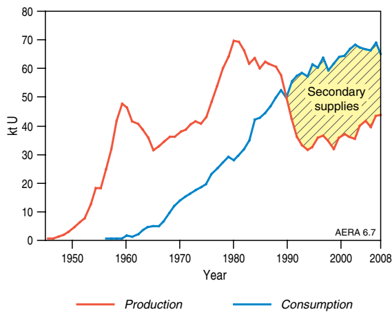
Figure 6.7 World uranium production and consumption for energy purposes Source: OECD/NEA-IAEA 2006, 2008, WNA 2009b, 2009c
