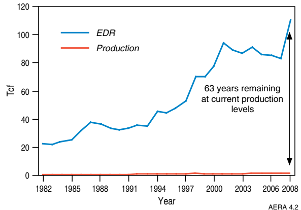
Figure 4.2 Conventional gas resources and production Source: Geoscience Australia 2009
