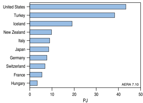
Figure 7.10 World direct use of geothermal energy, major countries, 2007
