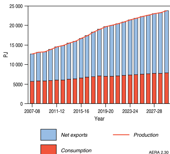
Figure 2.30 Australia's energy supply-demand balance, excluding uranium, 2007–08 to 2029–30
