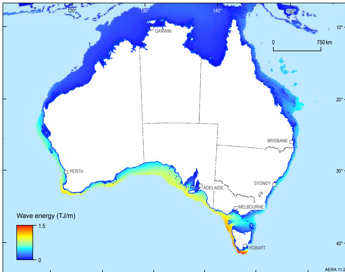
Figure 11.2 Total annual wave energy (in Terrajoules per metre, TJ/m) on the Australian continental shelf (less than 300 m water depth)
