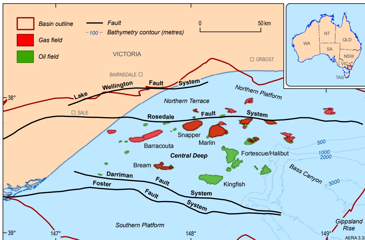
Figure 3.32 Gippsland Basin showing oil and gas fields and structural elements
