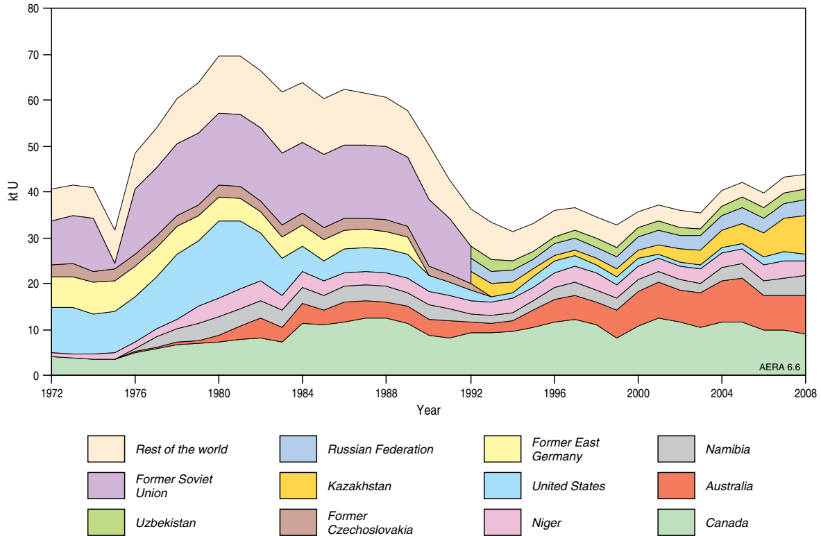
Figure 6.6 World uranium production, by major producer Source: OECD/NEA-IAEA 2006, 2008
