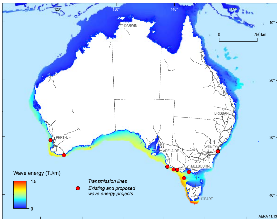
Figure 11.13 Total annual wave energy (TJ/m) on the Australian continental shelf (water depths less than 300 m) and wave energy projects. The total annual wave energy at each location represents an average of the 11 years from March 1997 to February 2008
