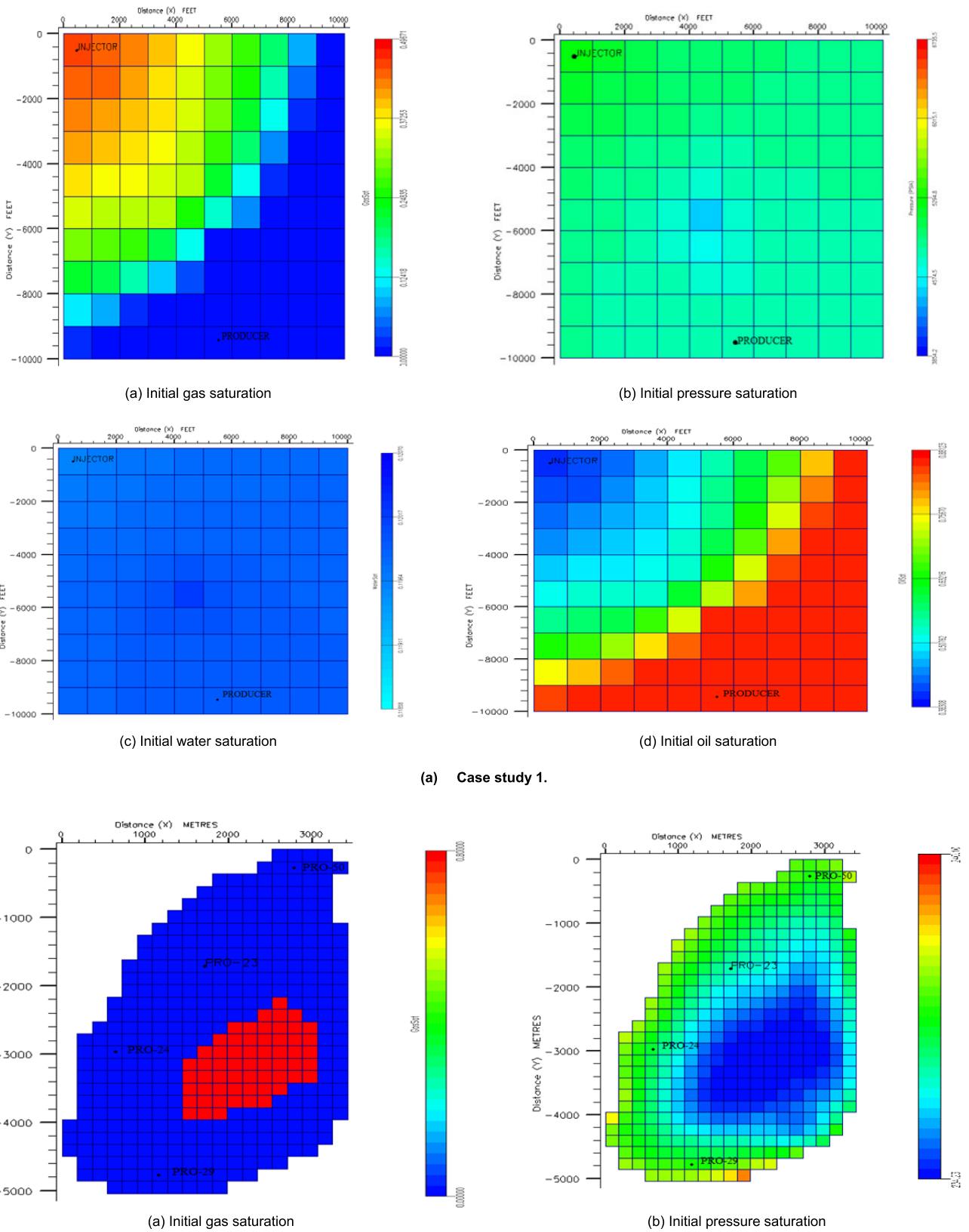
FIGURE 6. Initial pressure, oil, and gas saturation properties under different case studies [6].
