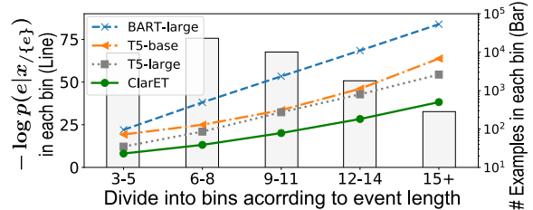
Figure 4: Event generation performance on the event-masked dev set (refer to Table 6) with event-length bins.
