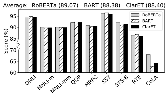
Figure 5: Fine-tuning results on GLUE dev, which verifies ClarET retains BART’s natural language understanding ability.
