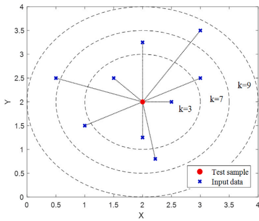
Fig. 10. An abstract model of the KNN algorithm.
