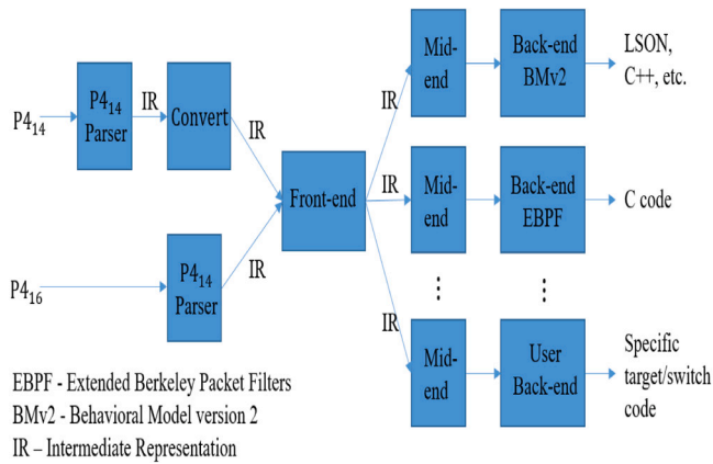
Fig. 9. Inside P4 compiler.
