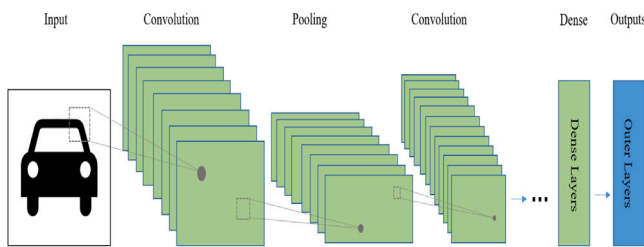
Fig. 18. An overview of training process of a convolutional neural network architecture.
