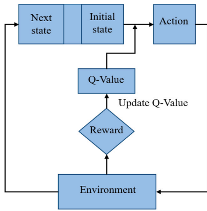
Fig. 13. An abstract view of Q-learning method, where every action taken in any state will be observed by the environment and generates a reward to provide insights about how good was the agent's action.
