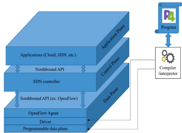
Fig. 7. P4 with OpenFlow architecture.
