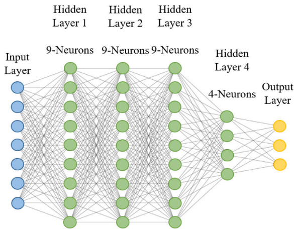
Fig. 17. The architecture of DNN.
