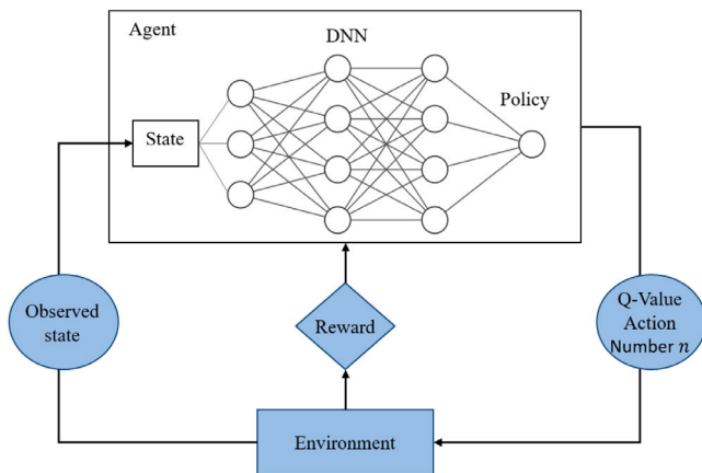
Fig. 14. The procedure of deep reinforcement learning.
