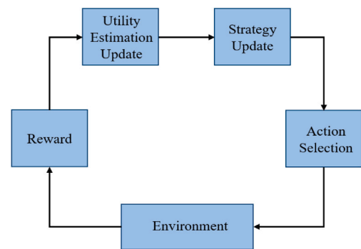
Fig. 16. Joint utility and strategy estimation-based learning process.
