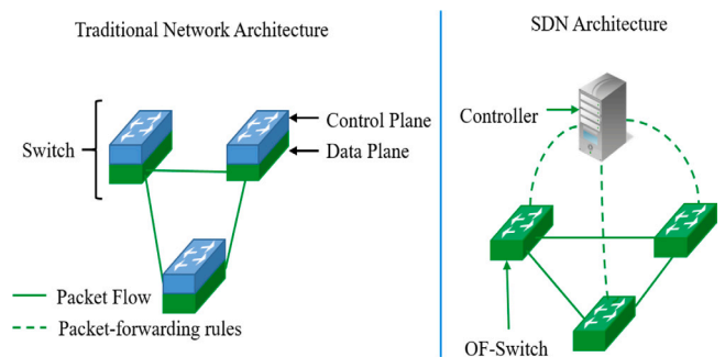
Fig. 4. Traditional network architecture versus SDN architecture.
