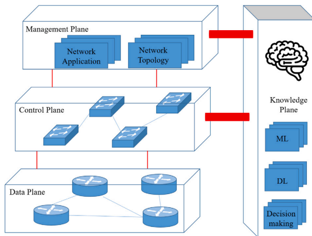
Fig. 5. KDN architecture.
