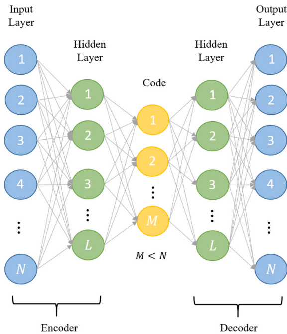
Fig. 20. Illustration of the structure of an autoencoder.
