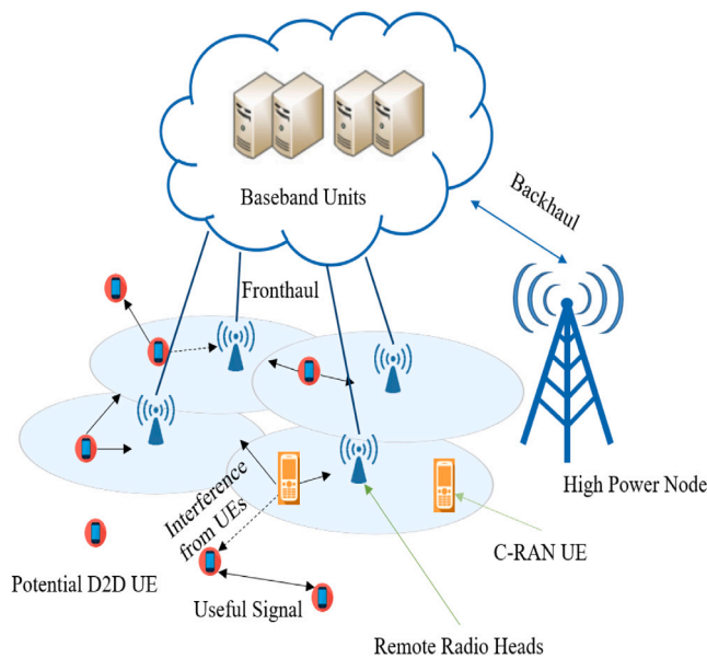
Fig. 21. An abstract system model of D2D enabled C-RAN.
