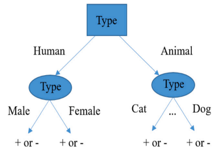
Fig. 11. An illustration of decision tree model to find out whether a person is overweighted.
