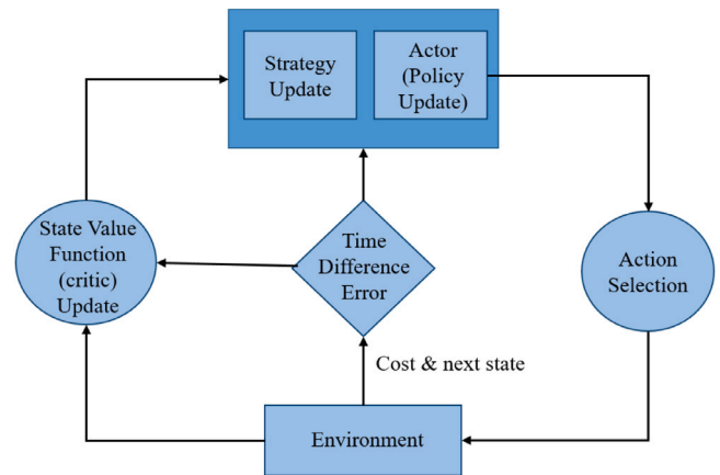
Fig. 15. An illustration of actor-critic learning algorithm.
