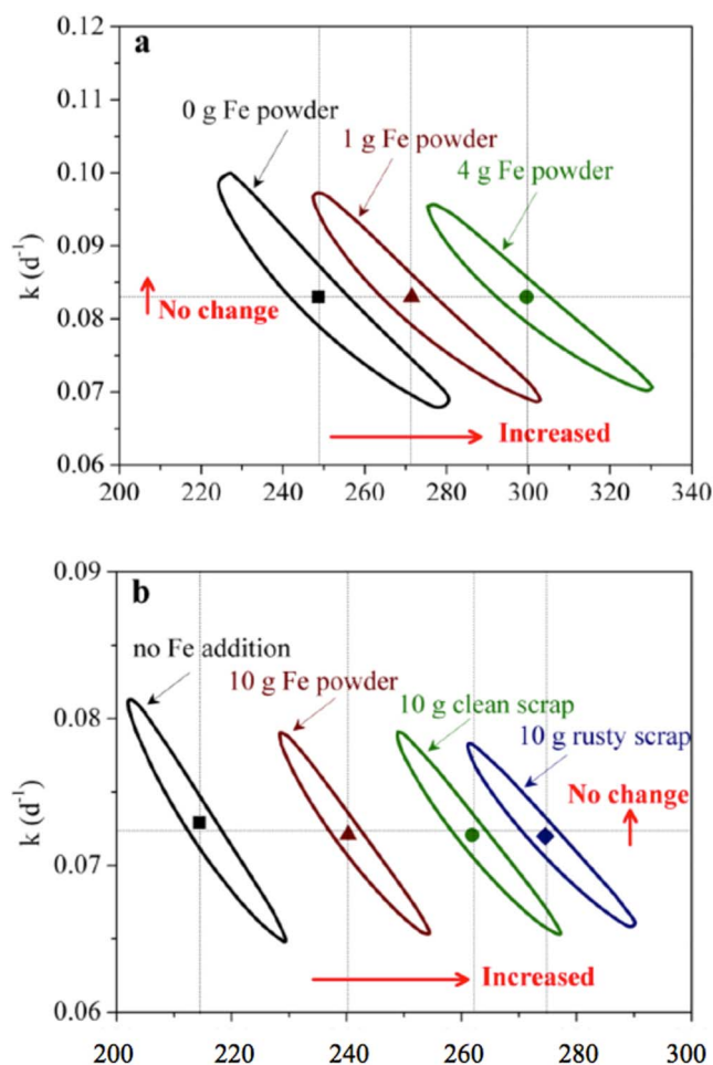
Figure 2 | The 95% confidence regions of the estimated hydrolysis rate ( k ) and biochemical methane potential ( B_0 ) with different ZVI additions: (a) using data from Experimental I; and (b) using data from Experiment II.
