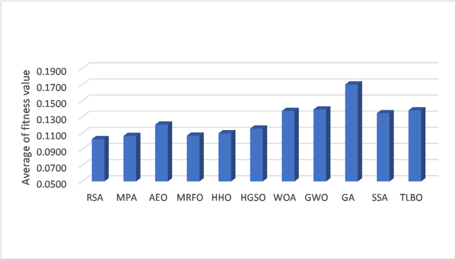
(b) Fitness
