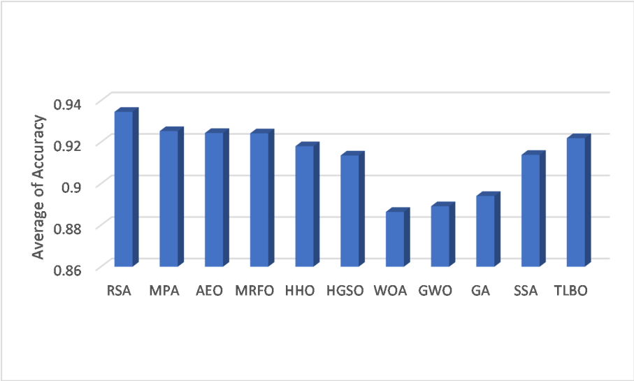
(a) Accuracy
