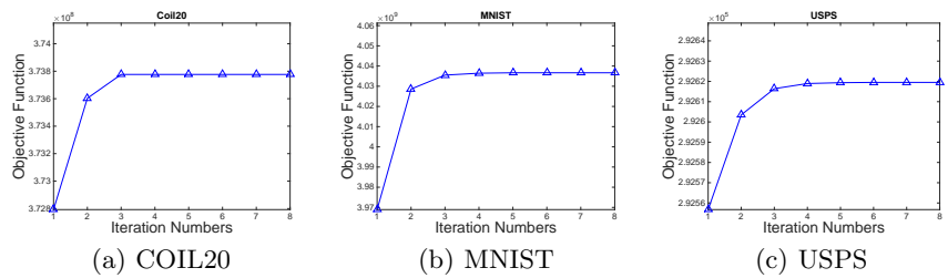
Fig. 5. Objective function values of our proposed objective function in (6) over three data sets, COIL20, MNIST, and USPS.
