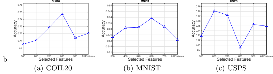
Fig. 1. Performance variation results with respect to the number of selected features using the proposed algorithm over three data sets, COIL20, MNIST, and USPS.
