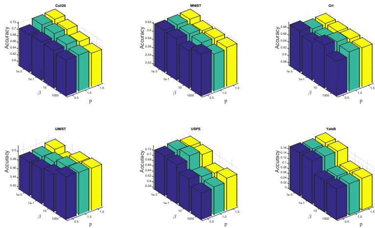
Fig. 4. Performance variation results under different combinations of \beta s and p s. \alpha is fixed at 10^{-1} .
