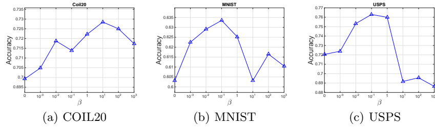
Fig. 2. Performance variation results with respect to different values of regularization parameter, \beta_s , over three data sets, COIL20, MNIST, and USPS.
