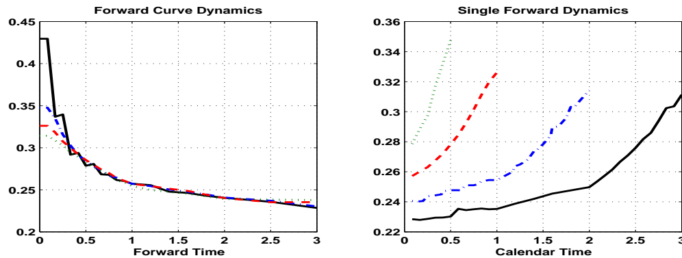
Figure 6: Left: Forward volatility structures at different calendar times (solid black = 0 (calibration date), dotted-dashed blue = 6 month, dashed red = 1 year, dotted green = 2 years). Right: Evolution of forward volatilities over lifetime (solid black = forward with 3 years maturity, dashed-dotted blue = 2 years, dashed red = 1 year, dotted green = 6 month).
