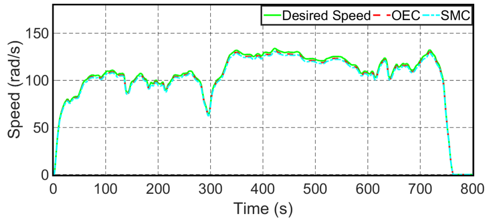
Figure 11. Experimental analysis: HWFET-based analysis at 60 °C.
