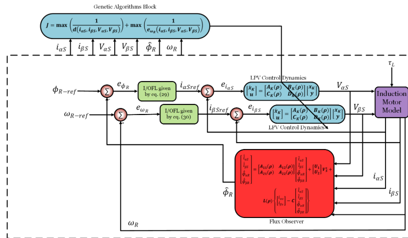
Figure 1. Optimized energy control scheme.
