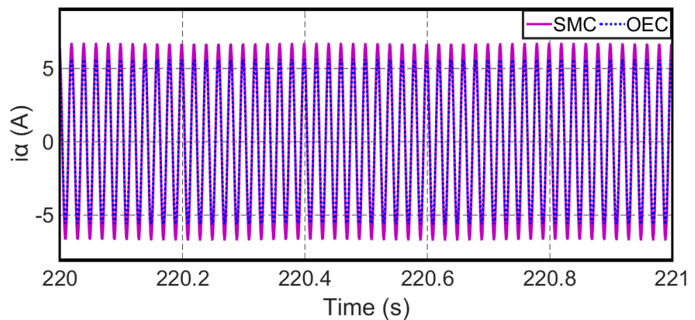
Figure 13. Experimental analysis: EV powertrain currents.
