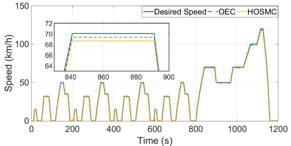
Figure 4. NEDC based analysis at 60 °C.
