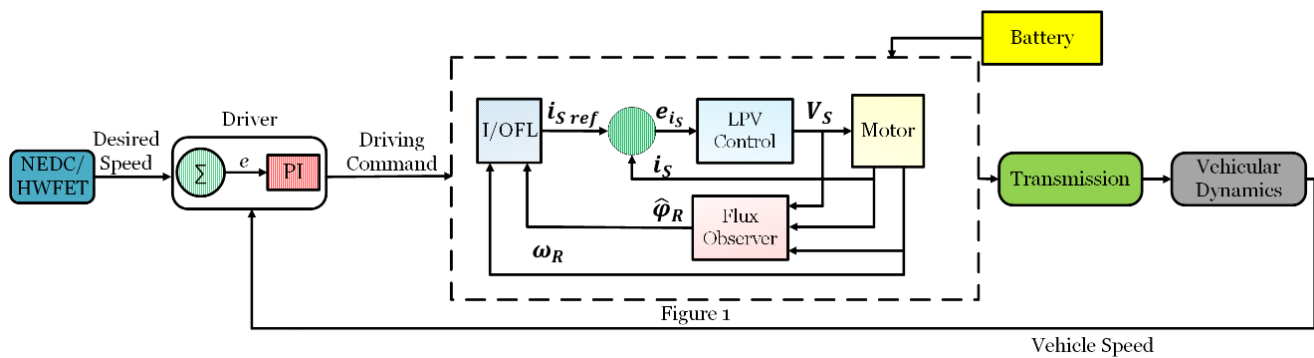
Figure 3. Electric vehicle control simulator.
