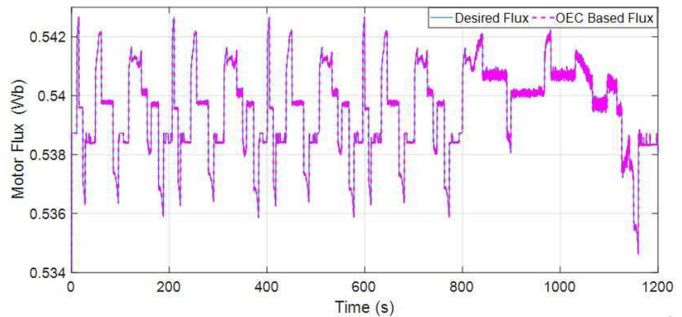
Figure 8. OEC-based flux tracking at 60 °C.
