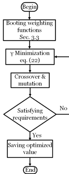
Figure 2. Controller synthesis through genetic algorithms.
