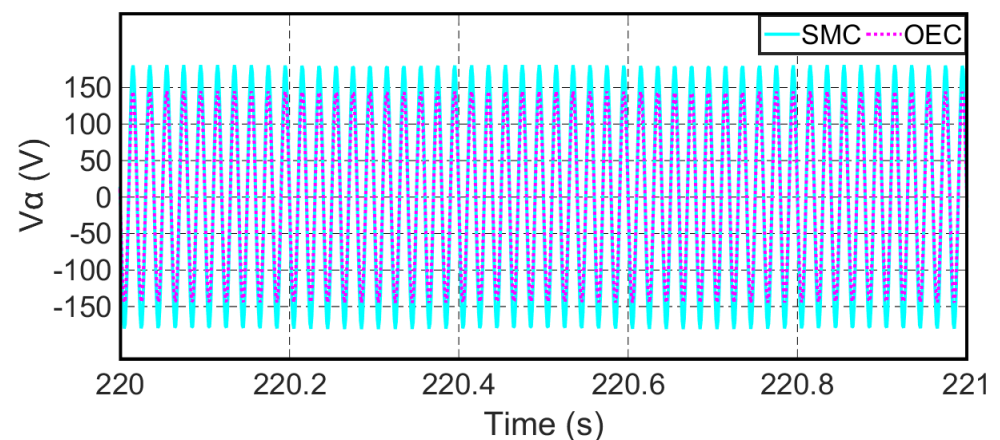
Figure 12. Experimental analysis: EV powertrain voltages.
