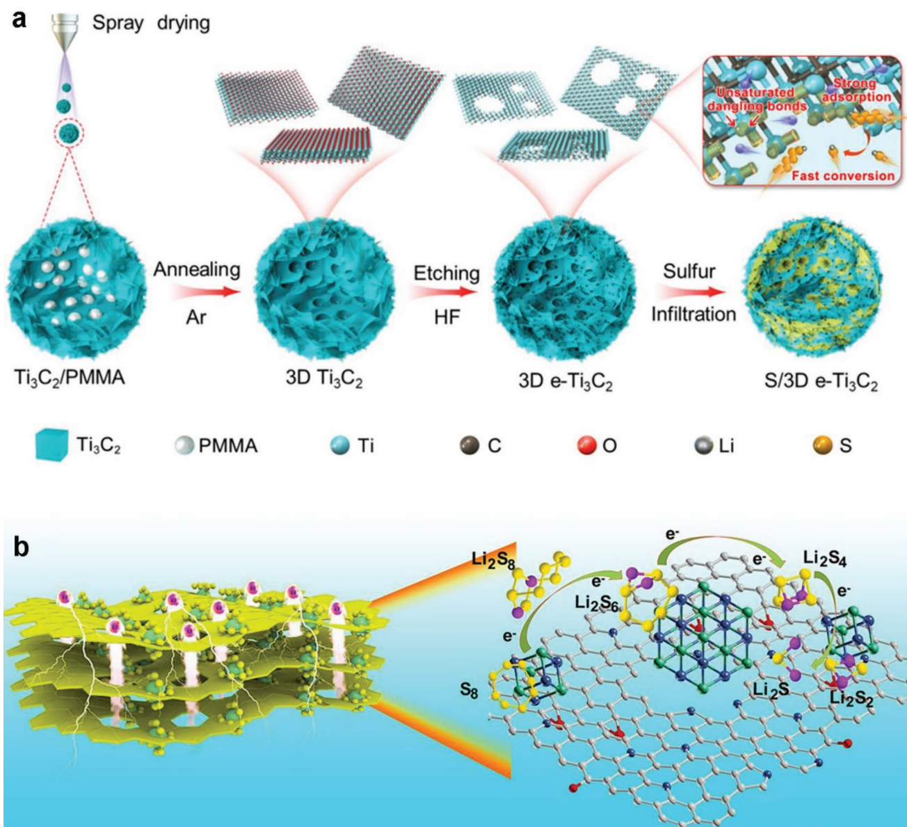
Figure 10. a) Schematic illustration of the fabrication of S/3D e-Ti 3 C 2 microspheres. Reproduced with permission. [123] Copyright 2021, American Chemical Society. b) VNQD–HG simultaneously promoting trapping, anchoring, and catalyzing sulfur species. Reproduced with permission. [129] Copyright 2021, American Chemical Society.
