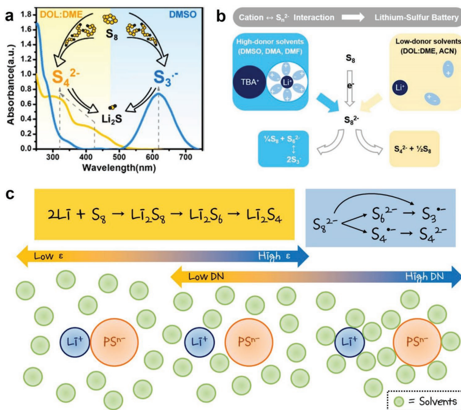
Figure 3. a) UV-vis spectra of S_4^{2-} and S_3^{\cdot-} radicals in DOL:DME (1:1) and DMSO. Reproduced with permission. [36] Copyright 2016, American Chemical Society. b) Summary of how polysulfide stability/speciation is affected by its interaction with cations and solvent molecules. Reproduced under the terms of the CC-BY license. [23] Copyright 2018, The Authors, Published by ECS. c) Schematic representation of solvent interaction with polysulfide species and the corresponding reduction reaction mechanisms in different solvent systems. Reproduced under the terms of the CC-BY license. [32] Copyright 2020, The Authors, Published by MDPI.
