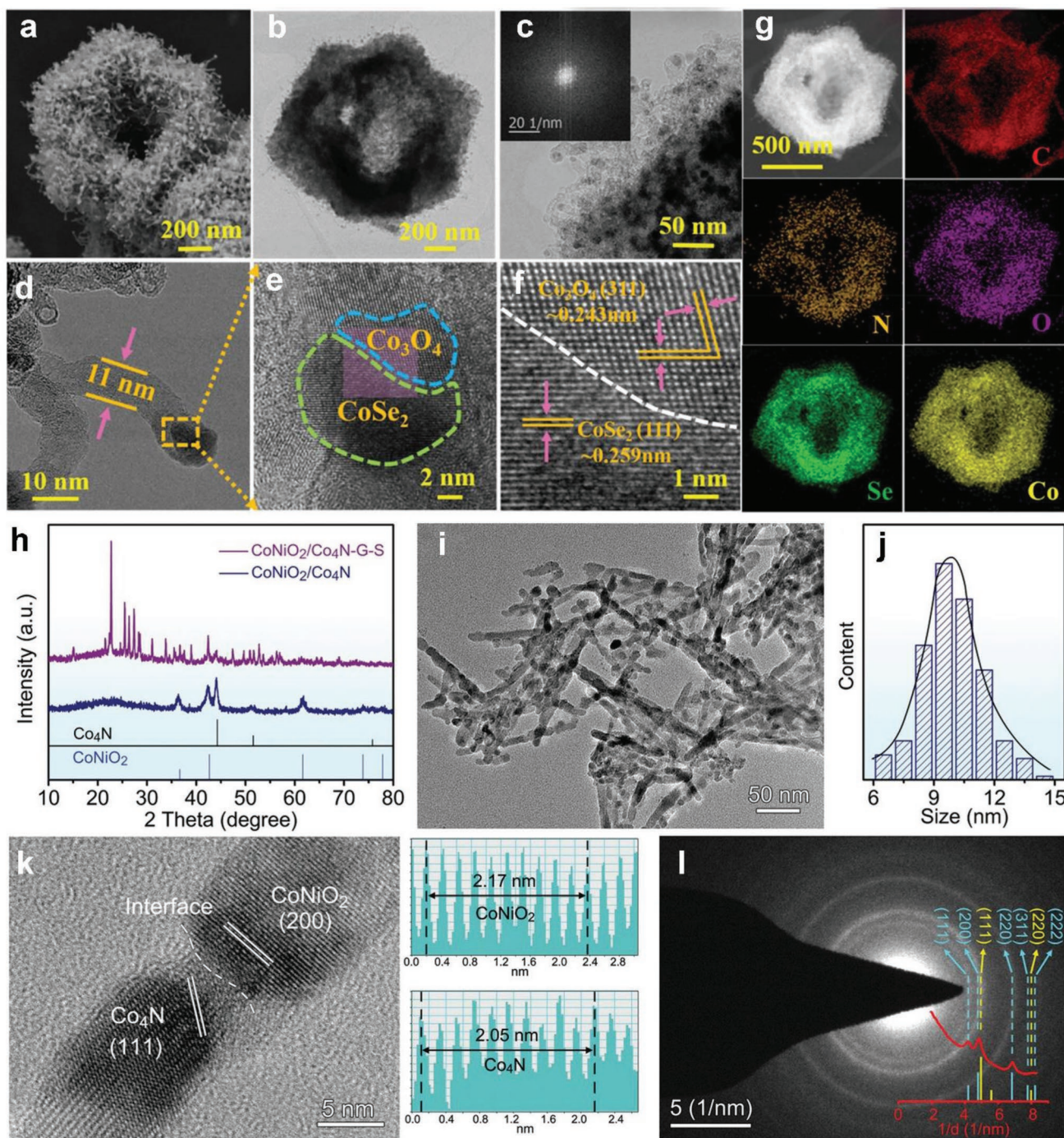
Figure 11. a) SEM image, b,c) TEM images, d–f) HRTEM image of the \text{CoSe}_2/\text{Co}_3\text{O}_4@\text{NC}-\text{CNT} heterostructure, g) scanning transmission electron microscopy (STEM) image and elemental mapping show the distribution of C, N, O, Se, Co, respectively. Reproduced with permission. [140] Copyright 2022, Wiley-VCH. h) XRD patterns. i,j) TEM image and diameter distribution. k) HRTEM result and the corresponding lattice spacing. l) SAED pattern and rotational integral. Reproduced with permission. [141] Copyright 2022, Wiley-VCH.
