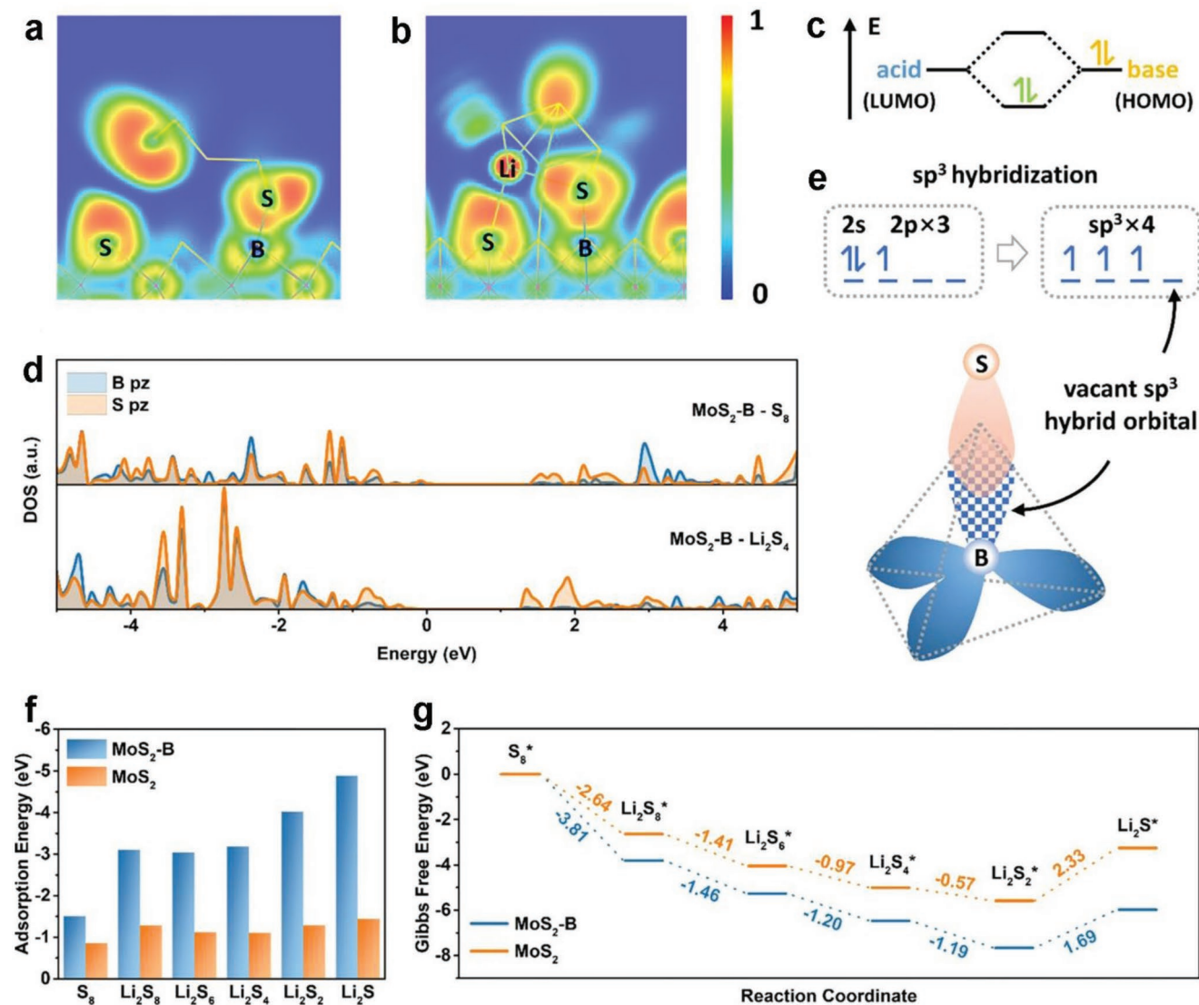
Figure 8. ELF plots of a) the MoS 2 -B-S 8 and b) the MoS 2 -B-Li 2 S 4 adsorption systems. c) Schematic representation of the Lewis acid-base interaction. d) DOS projected onto p z orbitals for the MoS 2 -B-S 8 and MoS 2 -B-Li 2 S 4 adsorption system. e) Schematic for the sp 3 hybridization of B in MoS 2 -B and the head-on orbital overlap between B and S. f) Adsorption energies of sulfur species and g) Gibbs free energy changes of sulfur reduction processes on MoS 2 -B and MoS 2 . Reproduced with permission. [102] Copyright 2021, American Chemical Society.
