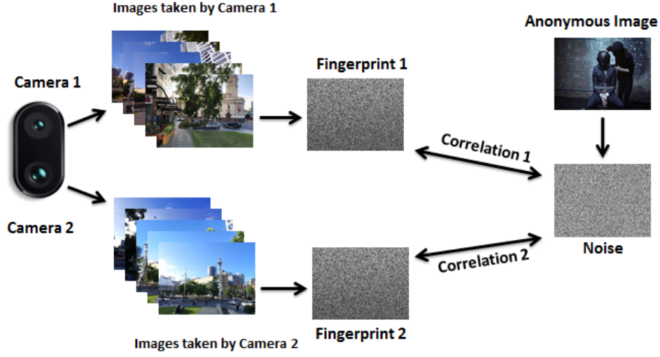
Figure 3: Multi-fingerprint verification process
