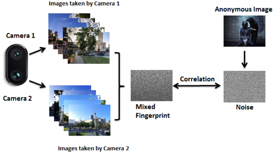
Figure 4: Mixed-fingerprint verification process
