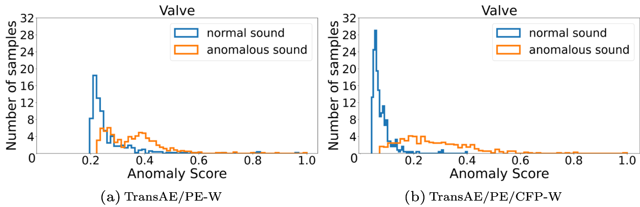
Fig. 7 The comparison between TransAE/PE-W and TransAE/PE/CFP-W on histograms of anomaly scores distribution of Valve
