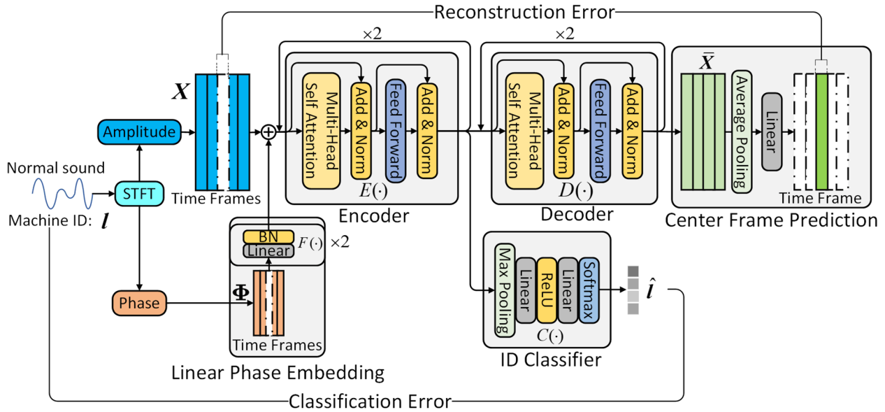
Fig. 3 The architecture of the proposed IDC-TransAE for normal sound reconstruction. \mathbf{X} and \Phi are the inputs to the model, which are obtained from the sound signal by removing the center frame. The final predicted center frame is obtained by average pooling of the output of the decoder \bar{\mathbf{X}} in frames and a linear layer, and \hat{\mathbf{I}} is the predicted machine ID probability of sound signal, which is obtained by max pooling of output of encoder \mathbf{z} in frames and two linear layers with softmax. IDC-TransAE is optimized by the combination of reconstruction error and classification error
