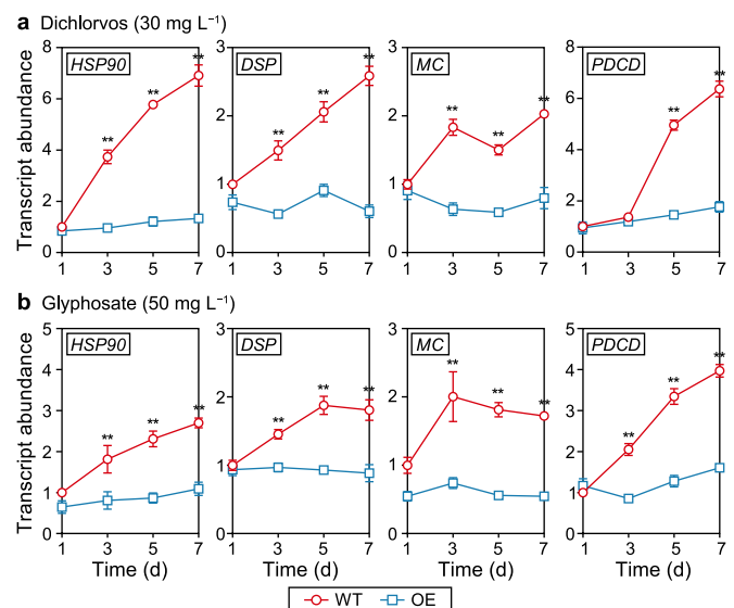
Fig. 7. Analyses of primary molecular markers of programmed cell death in P. tricornutum cultures throughout the cultivation period. a, Transcript abundances of HSP90 , DSP , MC , and PDCD genes in P. tricornutum cultures treated with 30 mg L -1 dichlorvos. b, Transcript abundances of HSP90 , DSP , MC , and PDCD genes in P. tricornutum cultures treated with 50 mg L -1 glyphosate. Each error bar represents the standard deviation of three samples. A significant difference (* p < 0.05 and ** p < 0.01) represents comparisons between the values of the WT and OE lines of P. tricornutum cultures.
