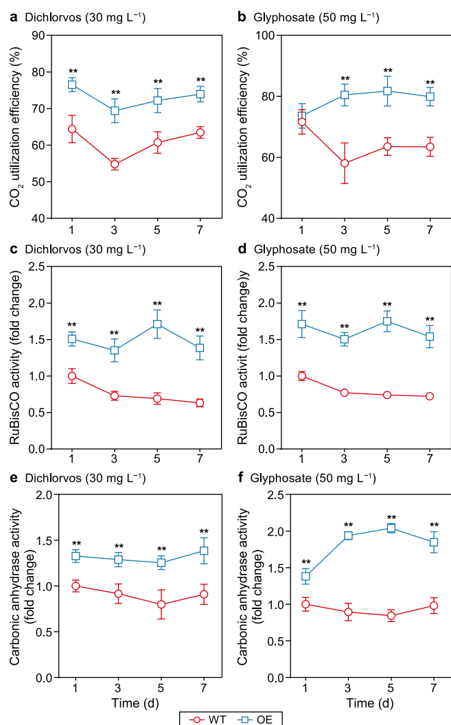
Fig. 3. a–b, Analyses of the CO 2 utilization and photosynthetic enzymes of P. tricornutum cultures throughout the cultivation period. CO 2 utilization efficiency of P. tricornutum cultures treated with 30 mg L -1 dichlorvos (a) or 50 mg L -1 glyphosate (b). c–d, Enzymatic activity of ribulose-1,5-bisphosphate carboxylase-oxygenase (RuBisCO) in P. tricornutum cultures treated with 30 mg L -1 dichlorvos (c) or 50 mg L -1 glyphosate (d). e–f, Enzymatic carbonic anhydrase activity in P. tricornutum cultures treated with 30 mg L -1 dichlorvos (e) or 50 mg L -1 glyphosate (f). Each error bar represents the standard deviation of three samples. A significant difference (* p < 0.05 and ** p < 0.01) represents comparisons between the values of the WT and OE lines of P. tricornutum cultures.
