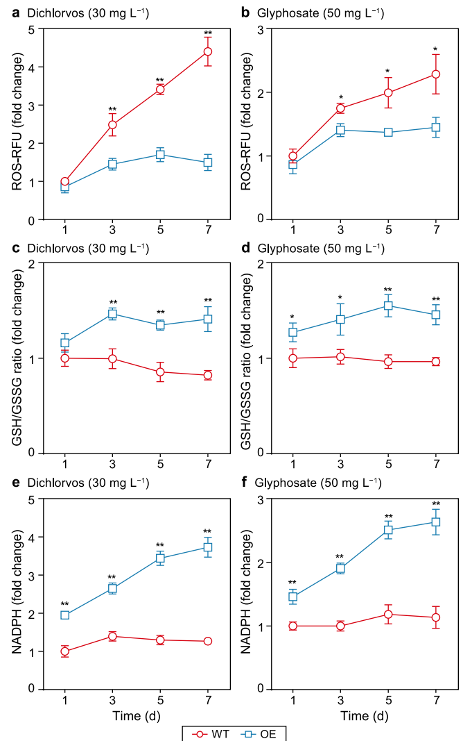
Fig. 5. a–b, Analyses of primary antioxidant markers of P. tricornutum cultures throughout the cultivation period. Relative ROS content of P. tricornutum cultures treated with 30 mg L -1 dichlorvos (a) or 50 mg L -1 glyphosate (b). c–d, The GSH/GSSG ratio of P. tricornutum cultures treated with 30 mg L -1 dichlorvos (c) or 50 mg L -1 glyphosate (d). e–f, NADPH content of P. tricornutum cultures treated with 30 mg L -1 dichlorvos (e) or 50 mg L -1 glyphosate (f). Each error bar represents the standard deviation of three samples. A significant difference (* p < 0.05 and ** p < 0.01) represents comparisons between the values of the WT and OE lines of P. tricornutum cultures.
