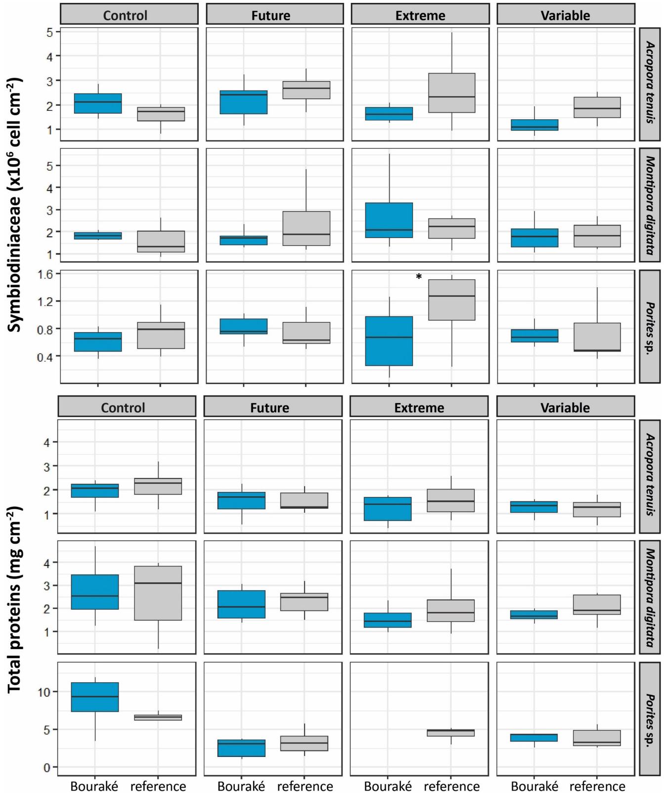
FIGURE 5 Symbiodiniaceae density and total protein content of corals from Bouraké (in blue) and the reference (in gray) site after 100 days of incubation at four pH conditions (Control, \text{pH}_{\text{NBS}} 8.11; Future, \text{pH}_{\text{NBS}} 7.76; Extreme, \text{pH}_{\text{NBS}} 7.54; and Variable, \text{pH}_{\text{NBS}} 7.56–8.07). Data are median \pm 25th and 75th percentiles ( n=6-8 , depending on species and pH condition). No data are available for the protein content of Porites sp. from Bouraké incubated at the Extreme pH condition. Asterisks indicate statistical significance at p < .05 ; see Table S7 for all post hoc comparisons.
