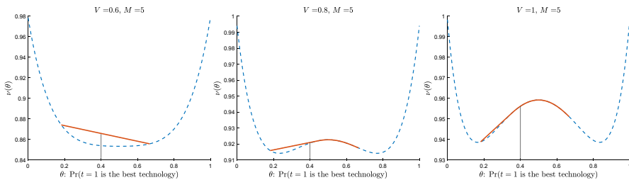
Fig. 6 Function v (dashed line) and its concavification \hat{v} (solid line) for f(x) = 1 - e^{-8x} , for different prize size. The vertical line indicates the fixed prior 0.4. The set of attainable posteriors with the experiment technology in Example 1 is \mathcal{P}_S = [0.18, 0.67]
