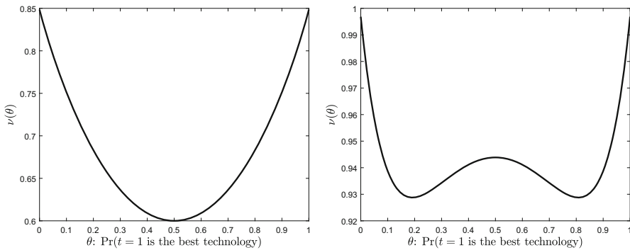
Fig. 3 Function v(\theta) , the value for the principal of inducing posterior \theta , for different functions f(\cdot) . Left panel: f(x) = \sqrt{x} ; Right panel: f(x) = 1 - \exp(-8x)
