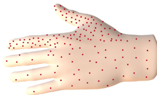
FIGURE 2 GSR is generally transferred in the V-shaped part of the hand between the thumb and the index finger (Meng & Caddy, 1997). GSR are mostly transferred on the upper part of the hand(s) holding the firearm but can also be transferred on the palm(s) as GSR are also present on the firearms.
