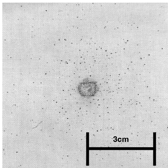
FIGURE 5 Visible GSR particles around a bullet hole on a white cotton tissue. The bullet was shot at 30 cm using a SigSauer P220 pistol (Thun® 9 mm Parabellum). This picture was provided by our colleague Julia Fischer
