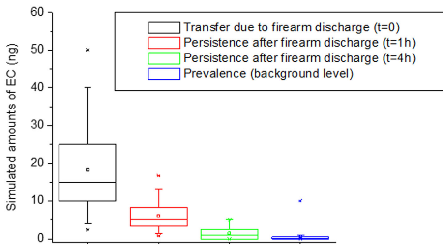
FIGURE 7 Simulated data for the transfer ( t = 0 h), the persistence ( t = 1 and 4 h), and prevalence of the stabilizer, the ethylcentralite (EC), on the hands of shooters and non-shooters based on available literature on the subject (Gassner et al., 2016; Hofstetter et al., 2017; Maitre et al., 2018; Manganelli et al., 2019)
