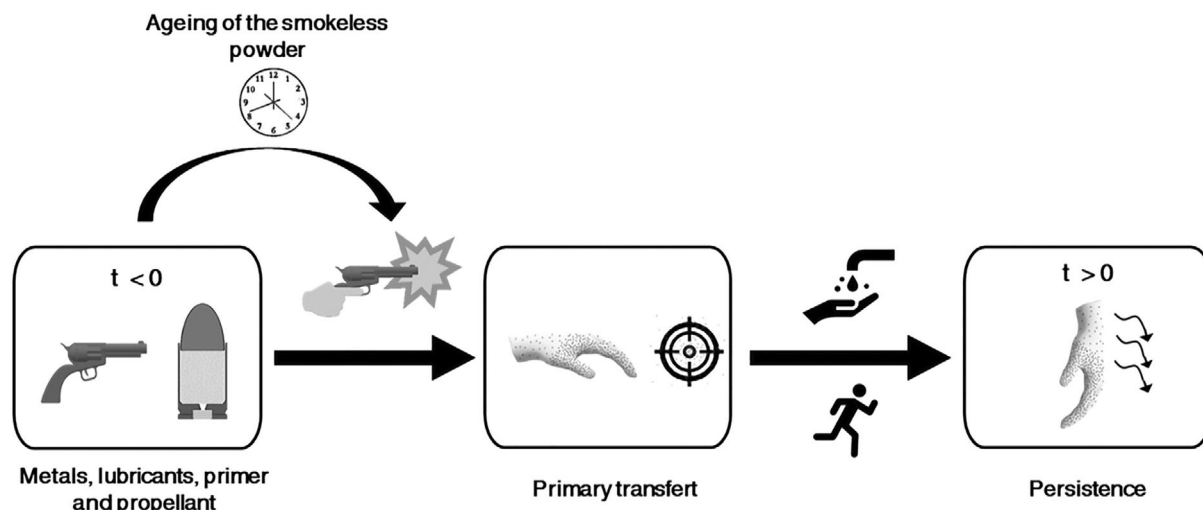
FIGURE 4 The GSR trace detected during the investigation of a firearm discharge is dependent: (1) on the state and composition of the initial materials used (e.g., firearm, ammunition) and on the age of the smokeless powder (e.g., depletion of the stabilizers/sensitizers), (2) on the transfer conditions (e.g., wind, distance to surrounding surfaces, receptor affinities), and (3) on the time, environment and activities between transfer and collection (e.g., rain or handwashing will strongly limit the persistence of GSR on the exposed surfaces)
