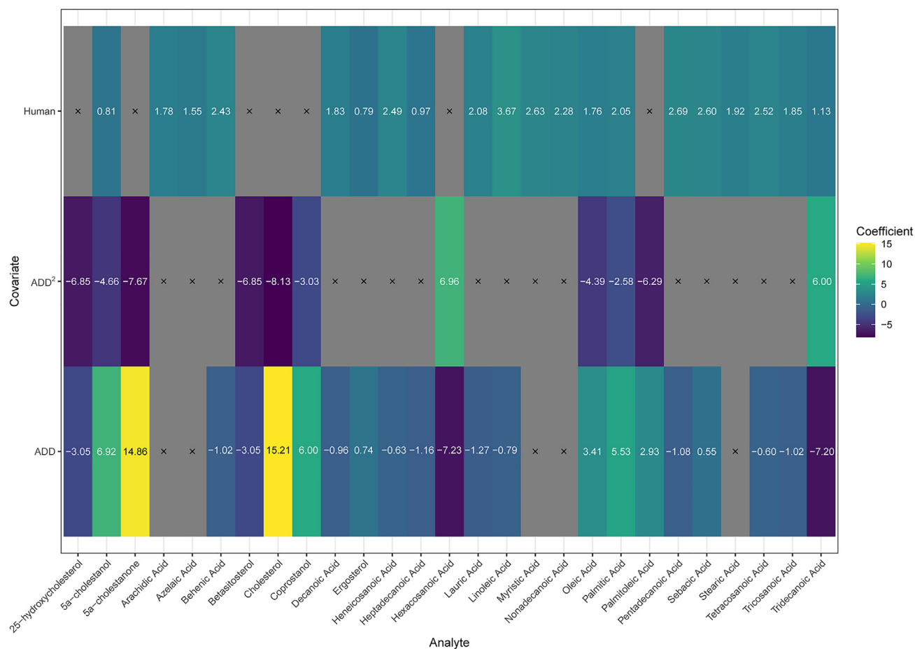
Figure 1. Matrix plot displaying the estimated fixed effects for the models fitted to the analytes
