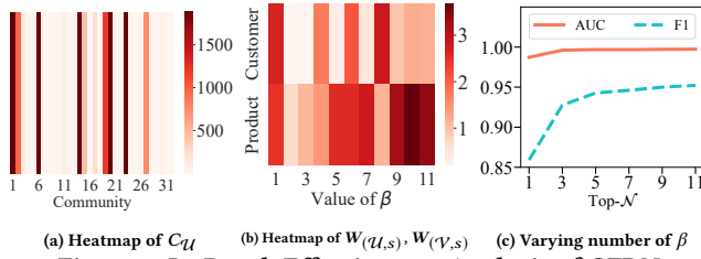
Figure 6: In-Depth Effectiveness Analysis of GFDN
