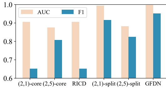
Figure 3: Comparison with Pattern-based Algorithms on TB
