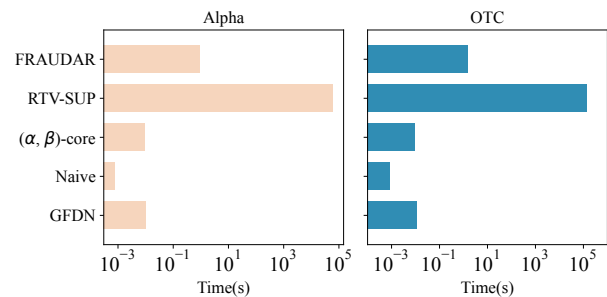
Figure 5: Query Time Evaluation of STARS
