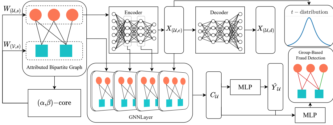
Figure 2: The Framework of GFND
