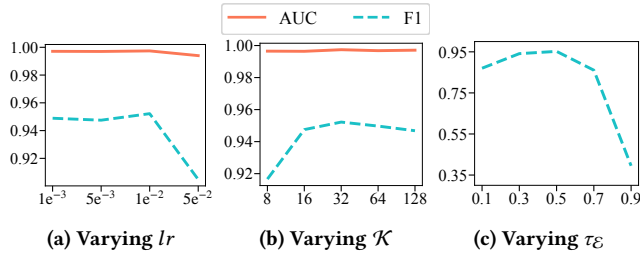
Figure 7: Parameter Analysis Results in GFDN
