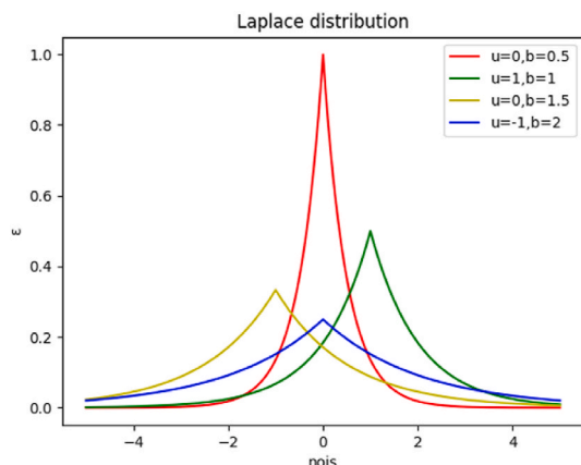
Fig. 7. Schematic of laplace distribution.
