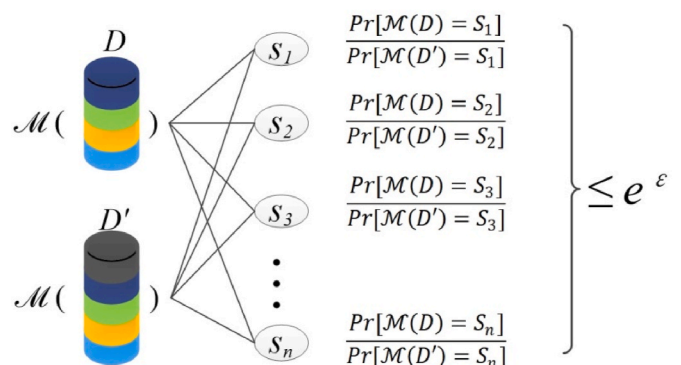
Fig. 6. Schematic of differential privacy.
