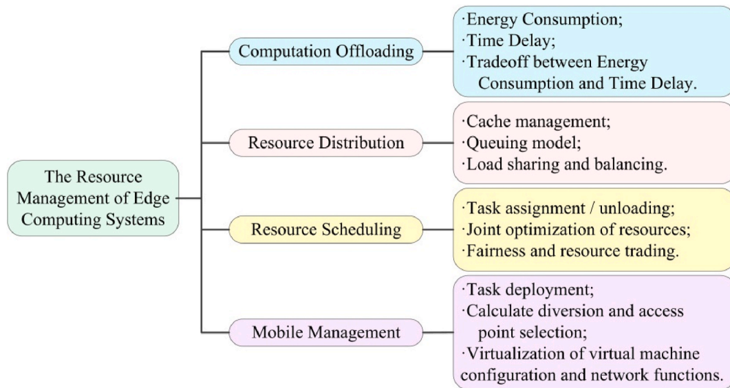
Fig. 12. The resource management of edge computing systems.
