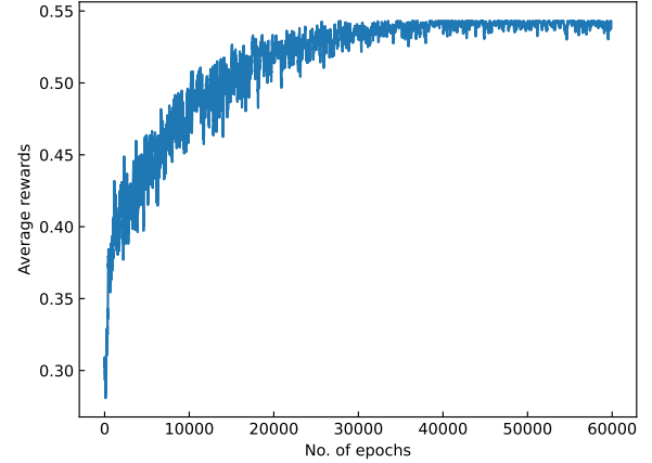
Fig. 8. Average rewards with a moving average value over the last 1000 steps.
