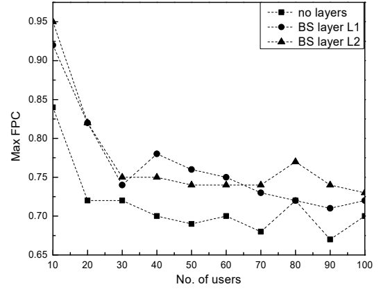
Fig. 6. FCM clustering performance for varying no. of users.
