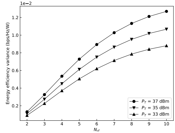
Fig. 11. The deviation of the energy efficiency value of the proposed scheme with respect to the full array gain scheme.
