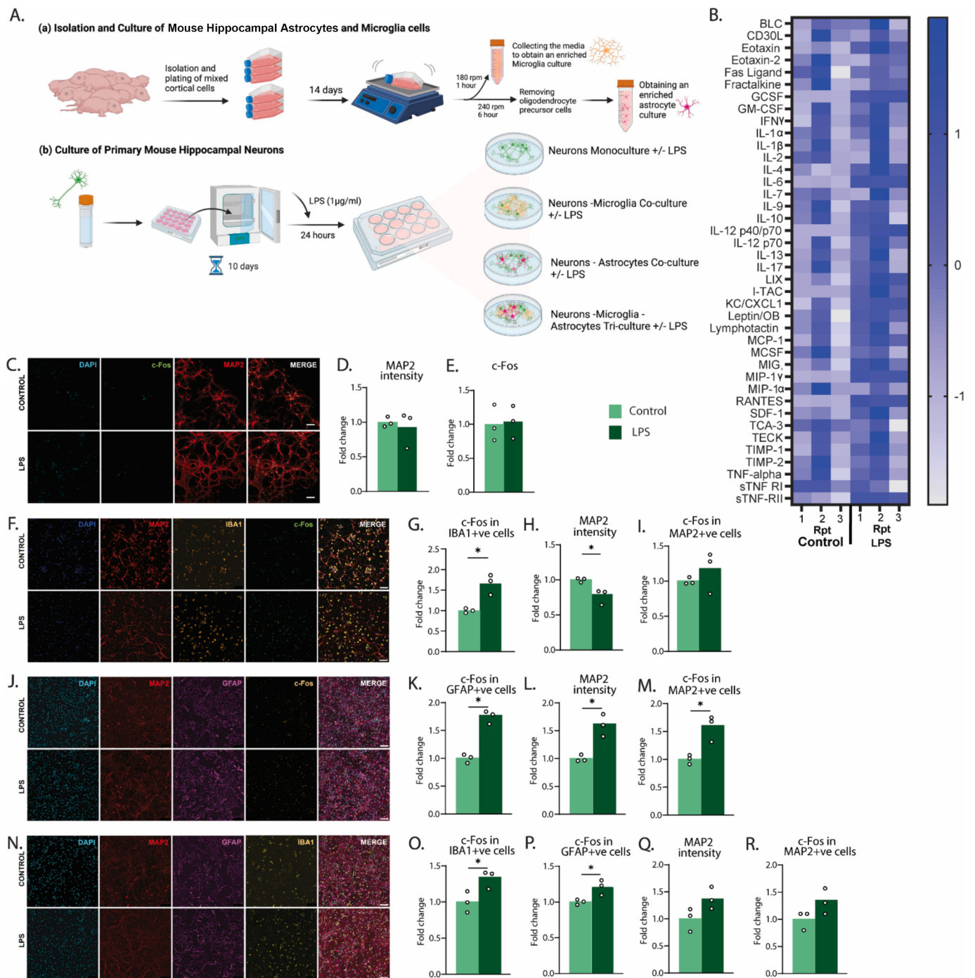
Fig. 1. Lipopolysaccharide application to primary cultures causes neuronal activation in the presence of astrocytes: (A) a) Schematic representation of the procedure for the collection and processing of mouse hippocampal microglia and astrocytes, and b) for mouse hippocampal neurons, for primary cell culture studies. Created with Biorender.com . (B) heatmap depicting fold change in protein expression of different cytokines from the untreated (control) and LPS-treated neuron, microglia, and astrocyte tricultures. (C,F,J,N) High resolution images showing saline and LPS treated cultures stained with DAPI-nucleus, MAP2-neurons, c-Fos-activated neurons, IBA1-microglia, GFAP-astrocytes (scale bar 100 \mu m) for: (C) neuronal monoculture; (F) neuron microglial coculture; (J) neuron astroglial coculture, (N) neuron microglia and astrocytes triculture. (D,E) Fold change of MAP2 and c-Fos intensity in control (light green) and LPS (dark green) treated neuronal monocultures. (G,H,I) Fold change of MAP2 and c-Fos intensity of neurons and c-Fos intensity of microglial cells in control (light green) and LPS (dark green) treated neuron microglial coculture. (K,L,M) Fold change of MAP2 and c-Fos intensity of neurons and c-Fos intensity of astrocyte cells in control (light green) and LPS (dark green) treated neuron astroglial coculture. (O,P,Q,R) Fold change of MAP2 and c-Fos intensity of neurons and c-Fos intensity of microglial and astrocytic cells in control (light green) and LPS (dark green) treated neuron microglia and astrocytes triculture. For each culture, n = 3 biological replicates (each technically replicated once). *p < 0.05 . (For interpretation of the references to colour in this figure legend, the reader is referred to the web version of this article.)
