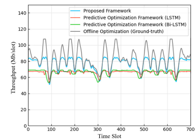
FIGURE 10. The admitted network traffic volume under Kaggle dataset.
