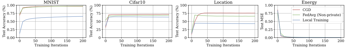
Figure 4: CGD's test accuracy compared to FedAvg and local training.
