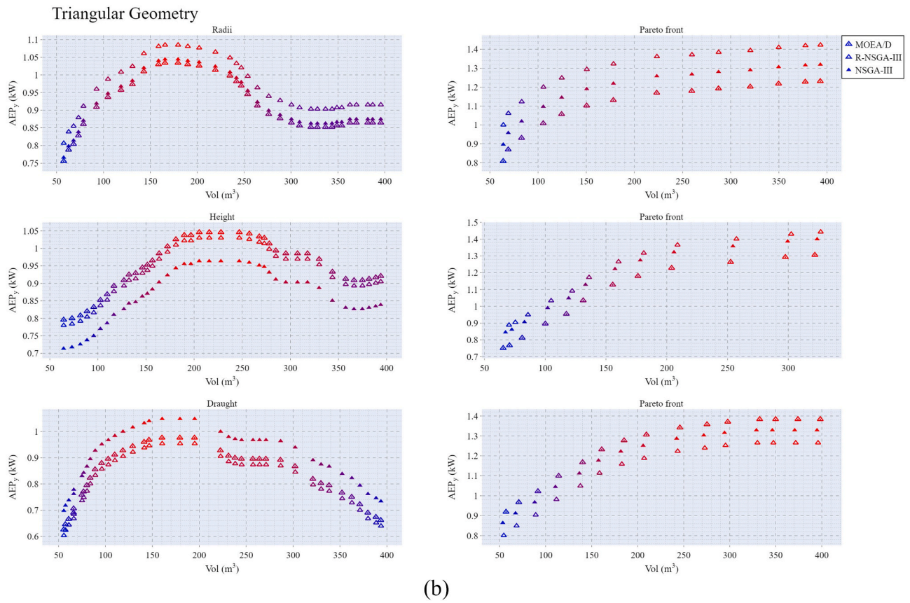
Fig. 14. AEP_y (left) and Pareto front (right) against the volume of (a) cylindrical, (b) triangular, (c) quadrilateral, and (d) octagonal geometries.
