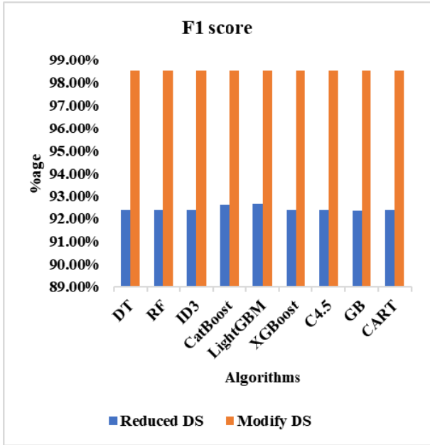
FIGURE 14. Comparison chart of F1 score of the DT and Its Variants – Before and after applying Feature Engineering.
