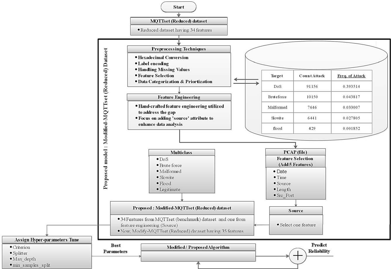
FIGURE 8. Proposed model: Modified MQTTset (Reduced) method of MQTTset dataset.
