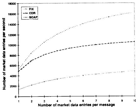
Figure 12: Throughput over 10 Mbps network
