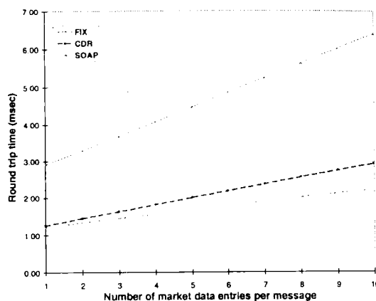
Figure 8: Round-trip times over 10 Mbps network
