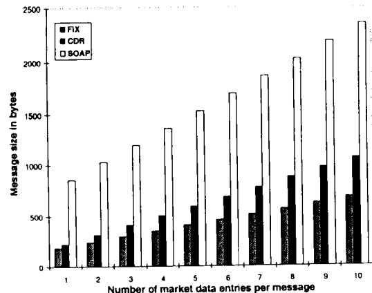
Figure 4: Message size comparison of the wire formats
