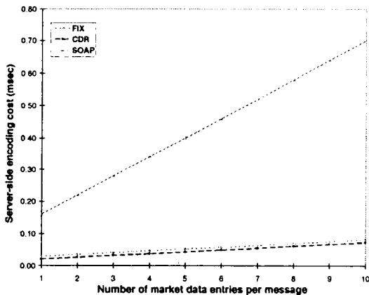
Figure 10: Server-side encoding costs
