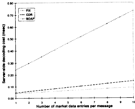
Figure 11: Server-side decoding costs
