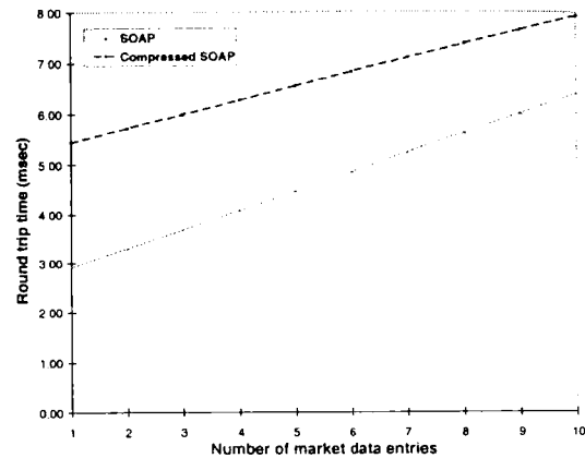
Figure 14: Round-trip times over 10 Mbps network for compressed and uncompressed SOAP messages
