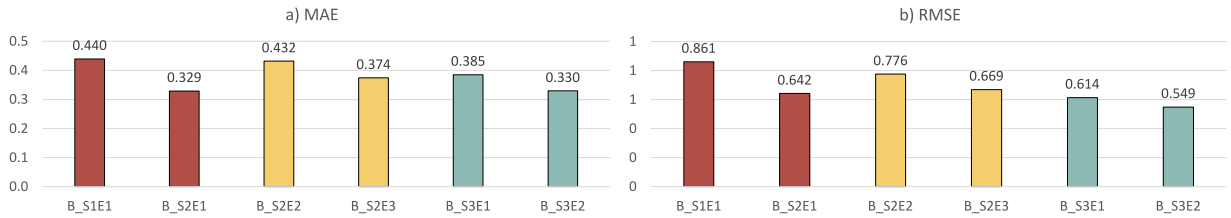
Fig. 7. Train networks errors evaluated between the ground truth and various estimated OD matrices when using: (a) MAE and (b) RMSE.
