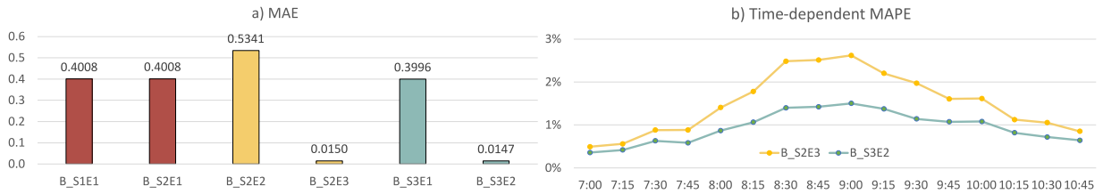
Fig. 6. (a) MAE errors for the bus networks evaluated between the ground truth and various estimated OD matrices and (b) Time-dependent MAPE evolution for our proposed entropy-weighted method (S3E2) versus the Hyman's method (S2E3).
