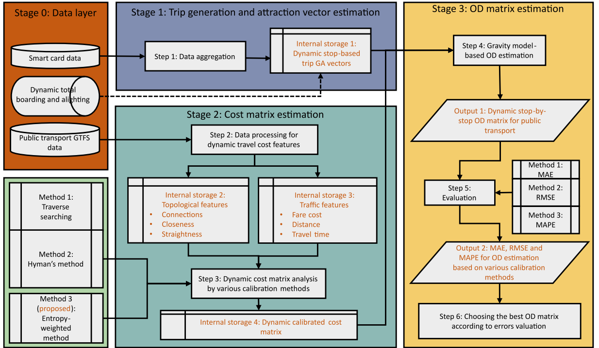
Fig. 1. Framework of our proposed dynamic stop-by-stop OD Estimation for a large-scale multi-modal PT network.
