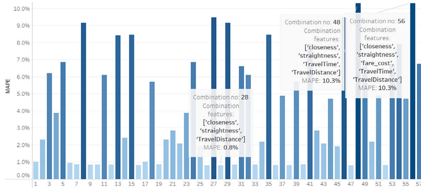
Fig. 5. MAPE error comparison for the combination of travel cost features in the train networks, fitted by an exponential function when using our proposed entropy-weighted method.
