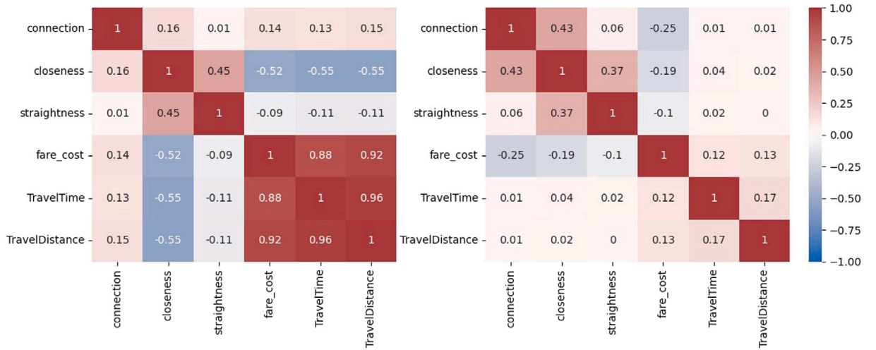
Fig. 4. Correlation matrices across six travel cost features for the bus networks (left) and the train networks (right).
