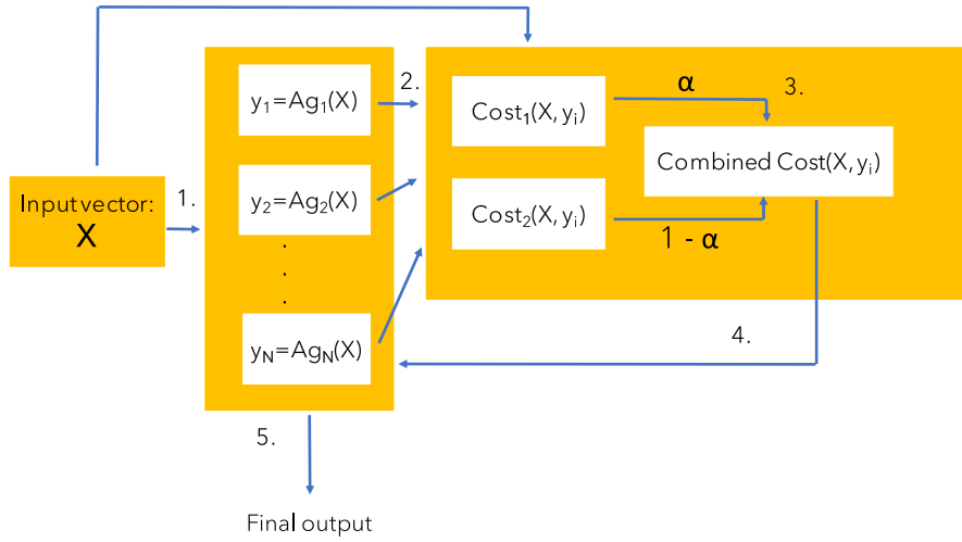
Fig. 3. Visual scheme for the MCA aggregation process. (In the case of the BCI framework in Fig. 1, X is the output of the LDA classifiers). 1. We compute all the possible aggregations. 2. We compute both cost functions for each aggregation output ( y_i ) with respect to the input vector. 3. We combine both costs for each aggregation with the mixing parameter \alpha . 4. We select the aggregation with the least cost value. 5. That aggregation is the final output of the MCA.
