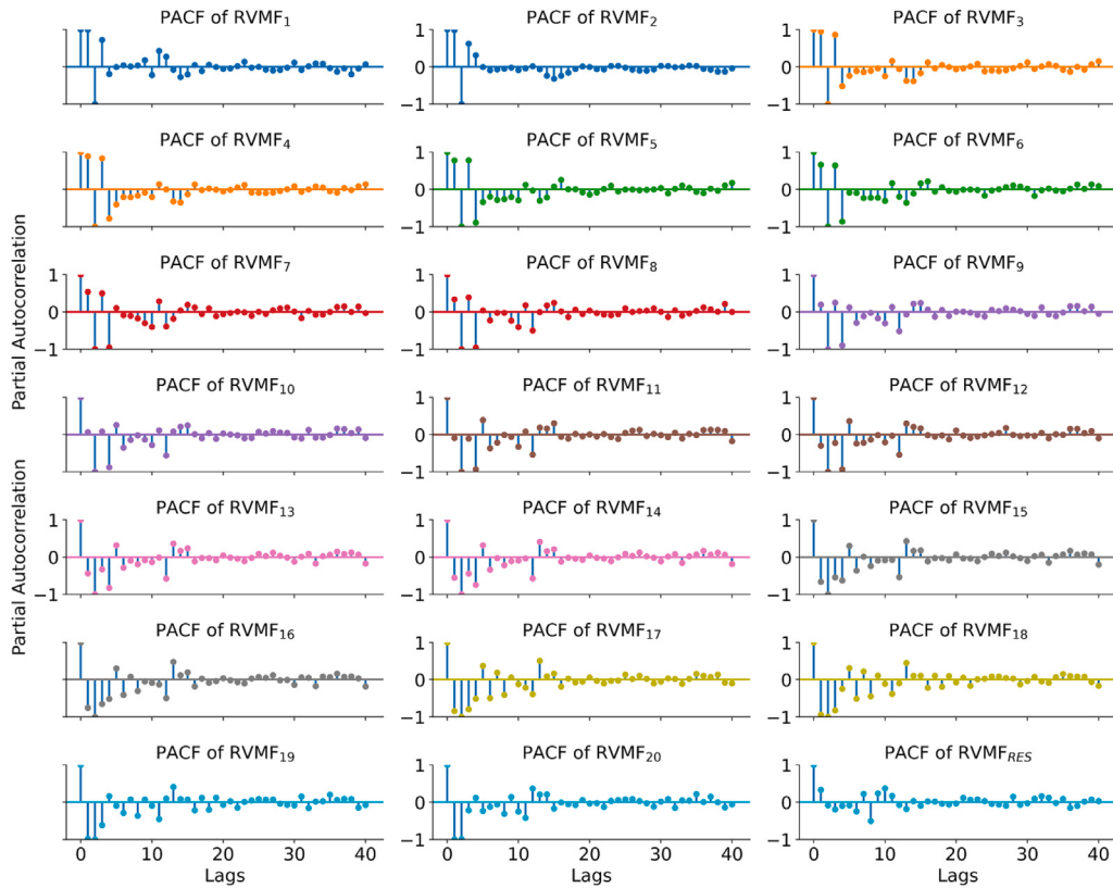
Fig. 6b. PACF of the decomposed residual series showing the most significant lags for the SA, where RVMF is the residual variational mode function.
