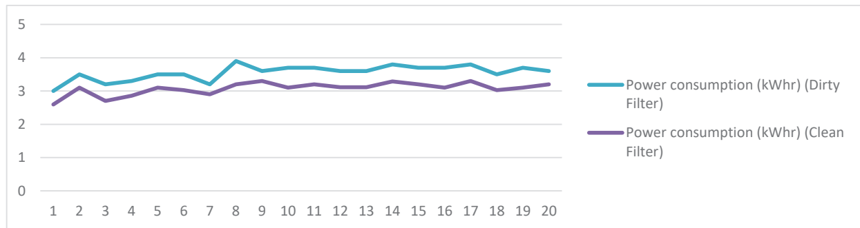
Fig 2: Comparison between power consumption with a dirty and a clean filter (each is operating for 8 hours a day for 20 days).
