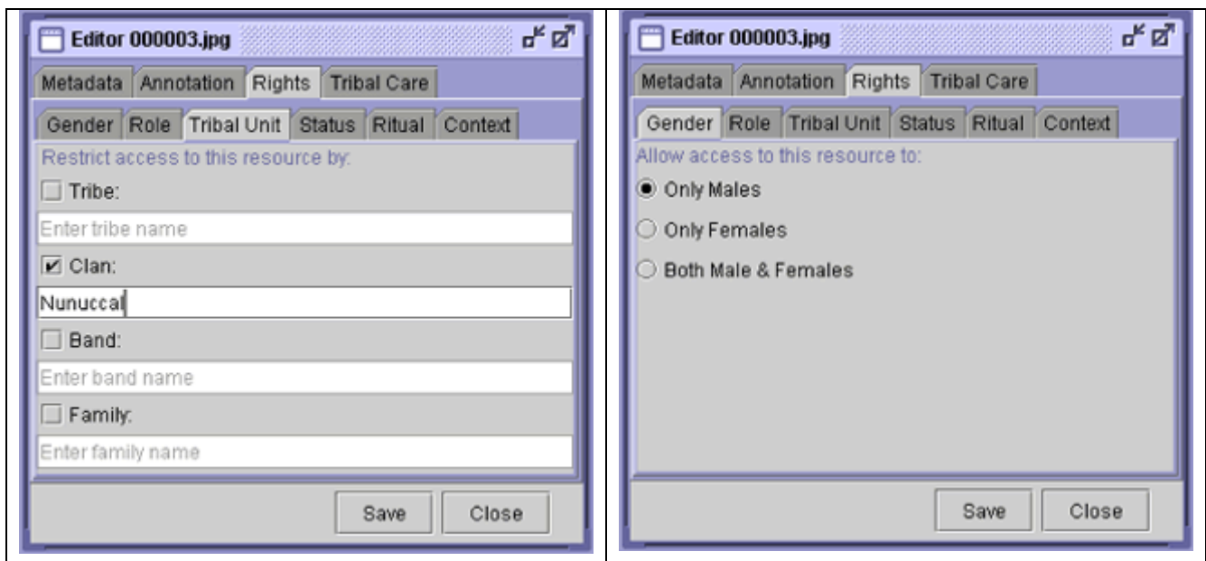
User Interface for Defining Access Restrictions which depend on the Users' Tribal Affiliation, Gender, Role and Status
