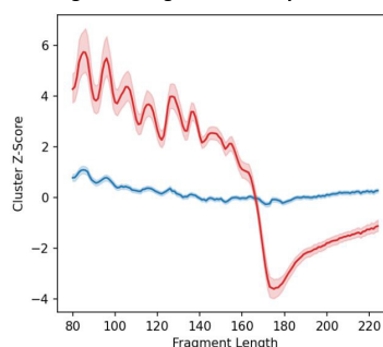
Fig. 4. Automated Gaussian mixture model clustering of cfDNA fragmentation signatures. (A) unsupervised AutoGMM clustering based on 12 principal components derived from variations in fragmentation patterns, including fragment end-positions, fragment lengths, and fragment end-motifs. (B) Strip plots illustrating the distribution of each principal component between clusters 1 and 2. Blue and red circles indicate the mean value for clusters 1 and 2, respectively. (C) Proportion of samples in each disease group assigned to Cluster 1 (blue) and 3 (red). (D–F) Mean fragment end-positions, fragment lengths, and fragment end-motif z-scores for samples in Cluster 1 (blue) and 2 (red). (F) Z-Scores are sorted based on the mean z-score in high tumor fraction cancers (IIA). Principal components and cluster assignment for all patients are provided in Dataset S5 .
